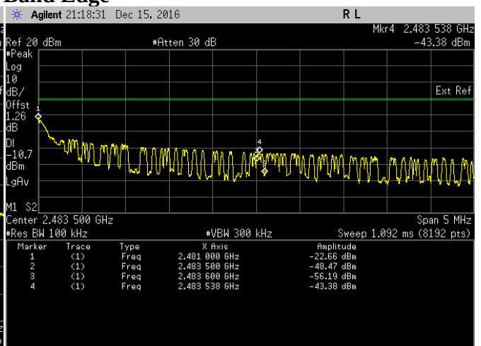
Band Edge. Bluetooth LE Frequency 2480 MHz Band Edge
