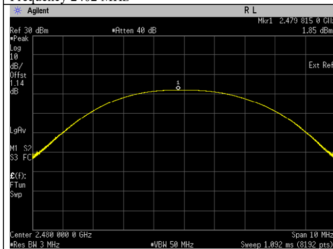
Frequency 2480 MHz
