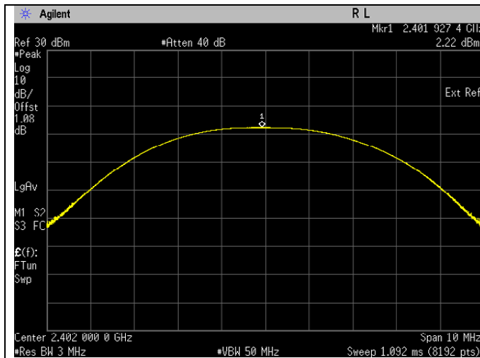
Frequency 2402 MHz
