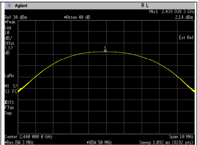
Frequency 2440 MHz
