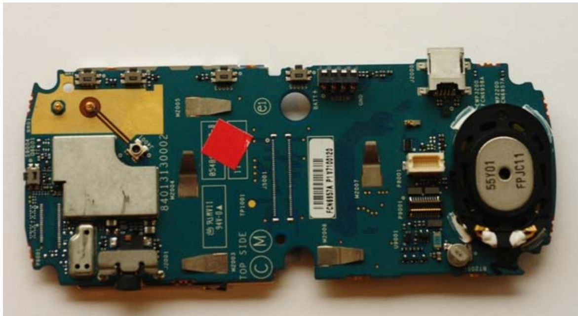
Photograph 3 – EWP2200 PCB Top View with Shields and Speaker
