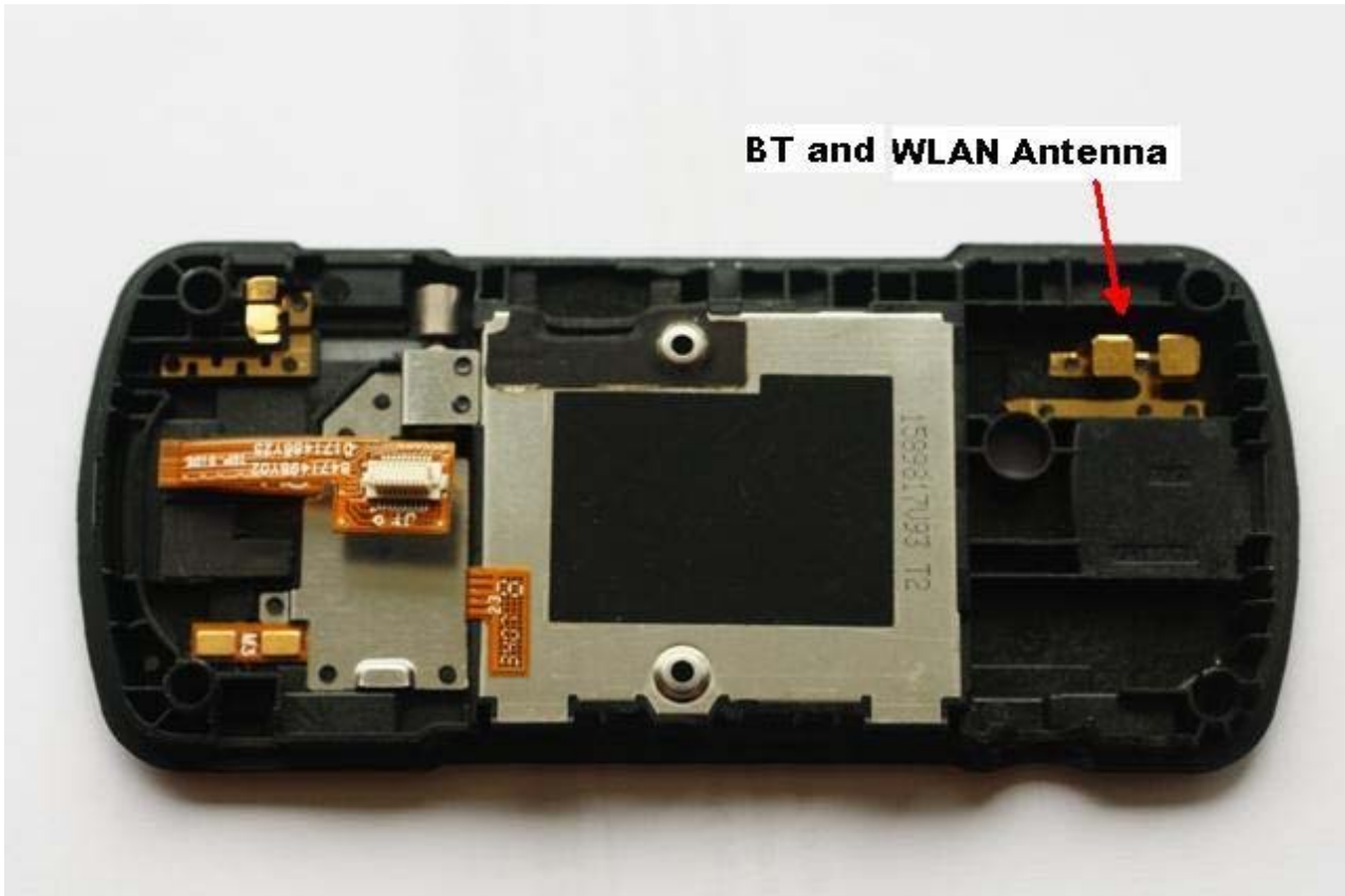
Photograph 8 – EWP2200 Antenna View
