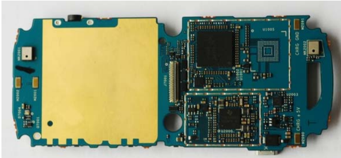
Photograph 6 – EWP2200 Bottom View with Shields and LCD removed
