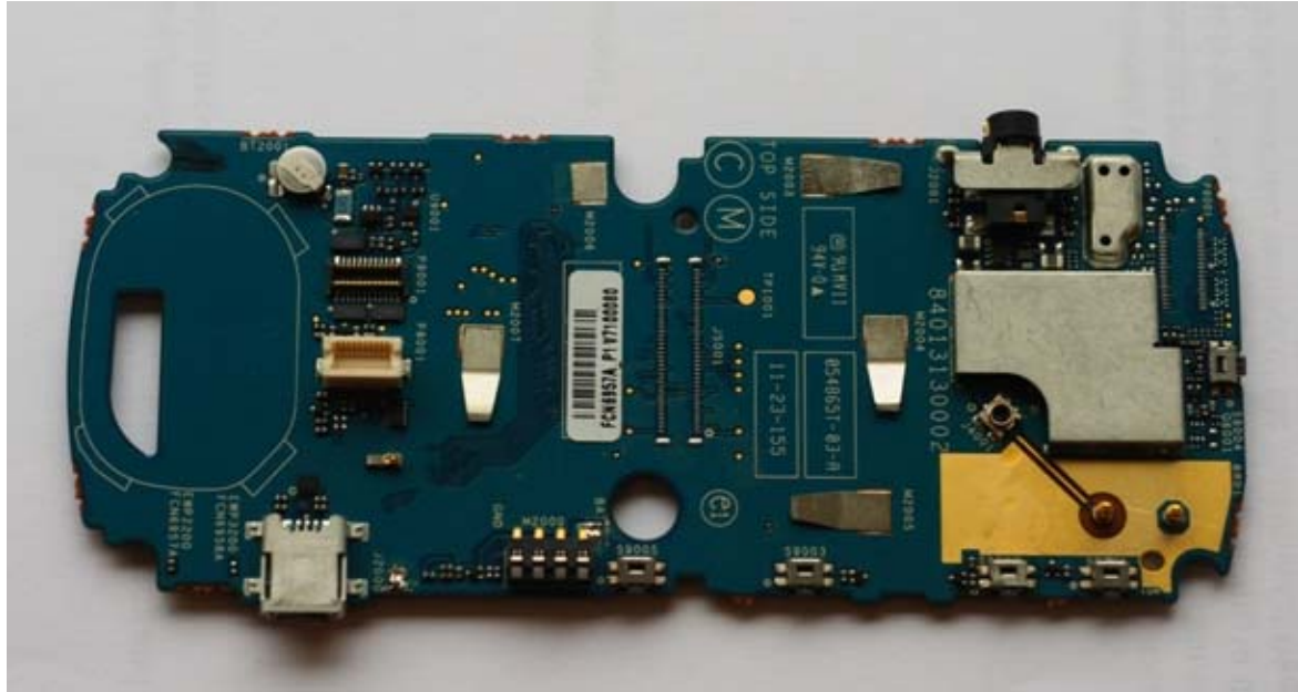
Photograph 2 – EWP2200 PCB Top View with Shields
