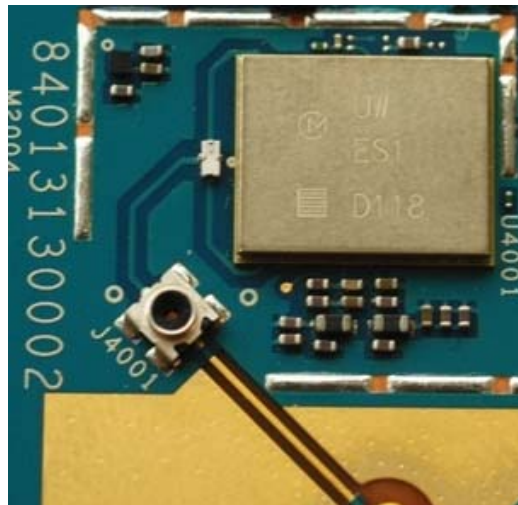
Photograph 7 – EWP2200 Transceiver (WLAN and BT)
