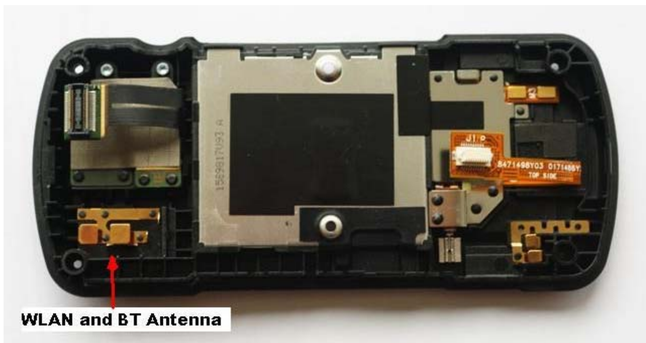
Photograph 7 – EWP3200 Antenna View
