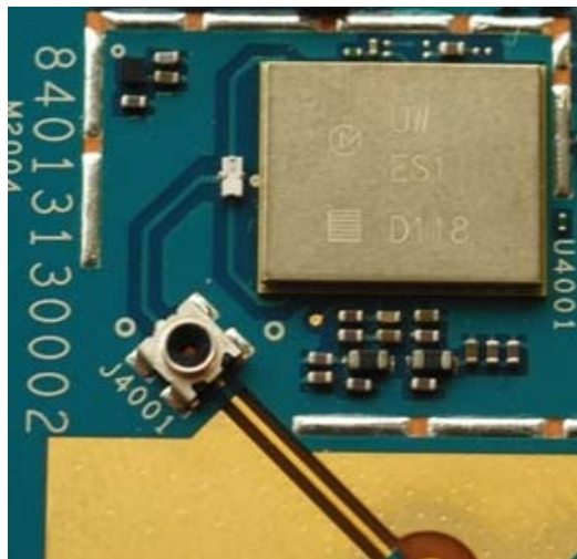
Photograph 6 – EWP3200 Transceiver (WLAN and BT)
