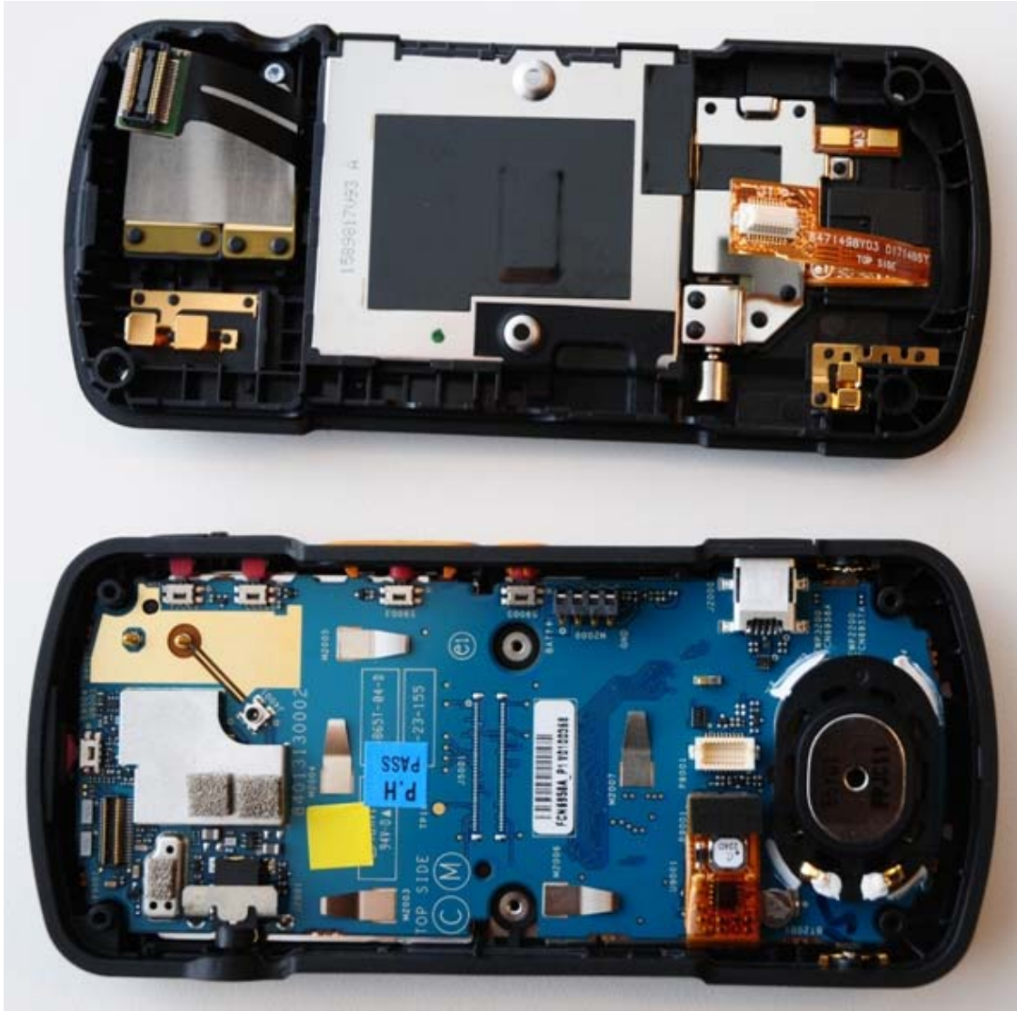
Photograph 1 – EWP3200 Opened with Shields
