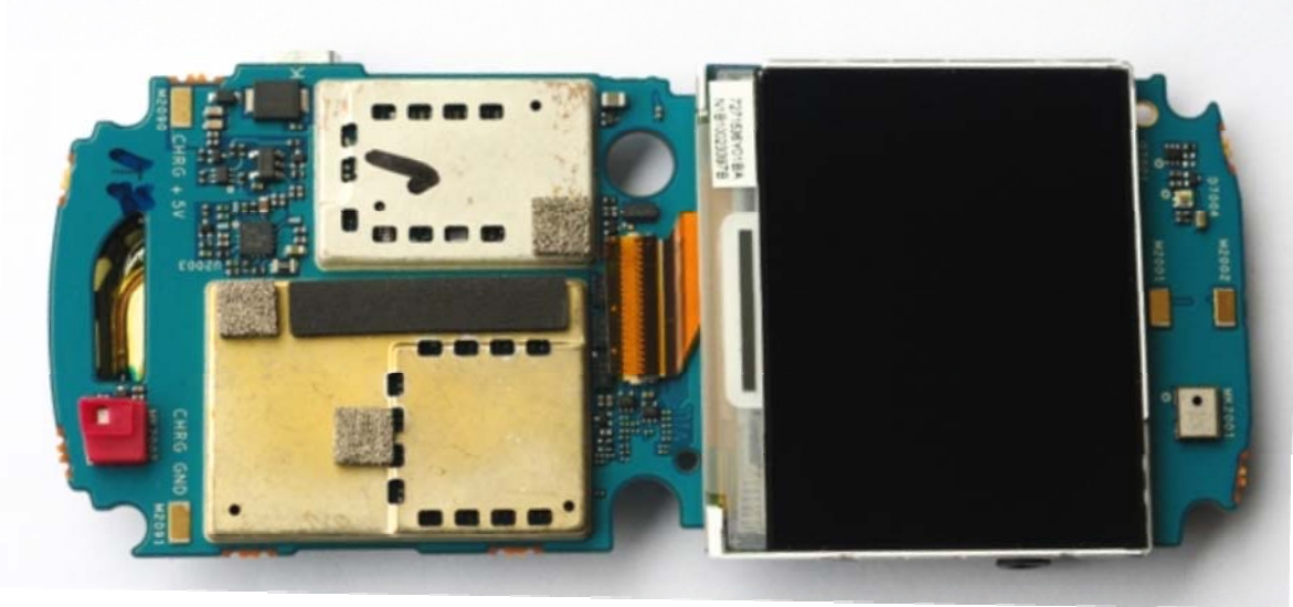
Photograph 4 – EWP3200 Bottom View with Shields and LCD
