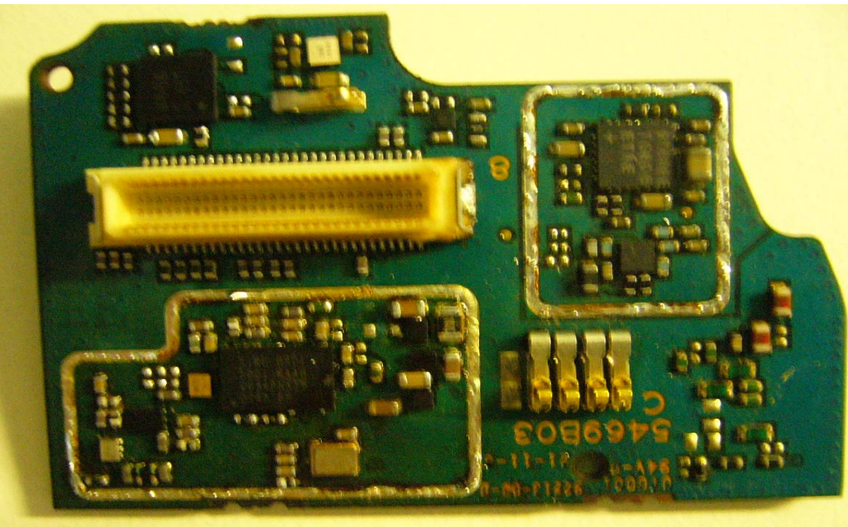
Expander board without shields board (Bottom)
