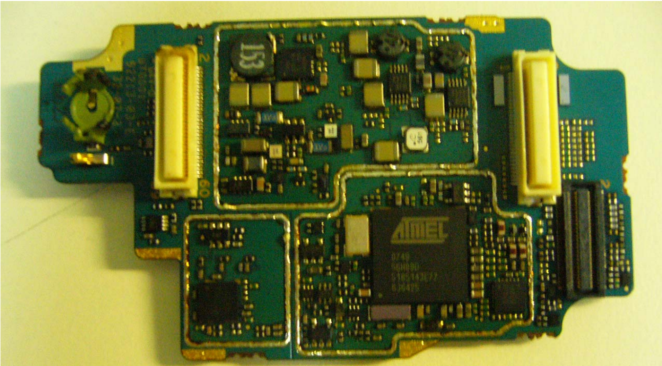
Vocon board without Shields (Top)
