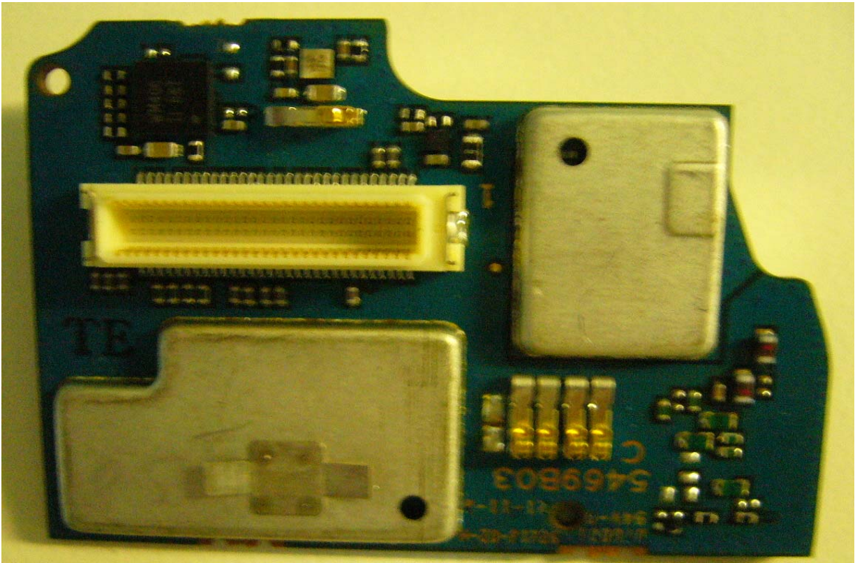
Expander board with shields board (Bottom)
