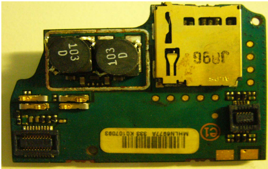
Expander board without shields board (Bottom)
