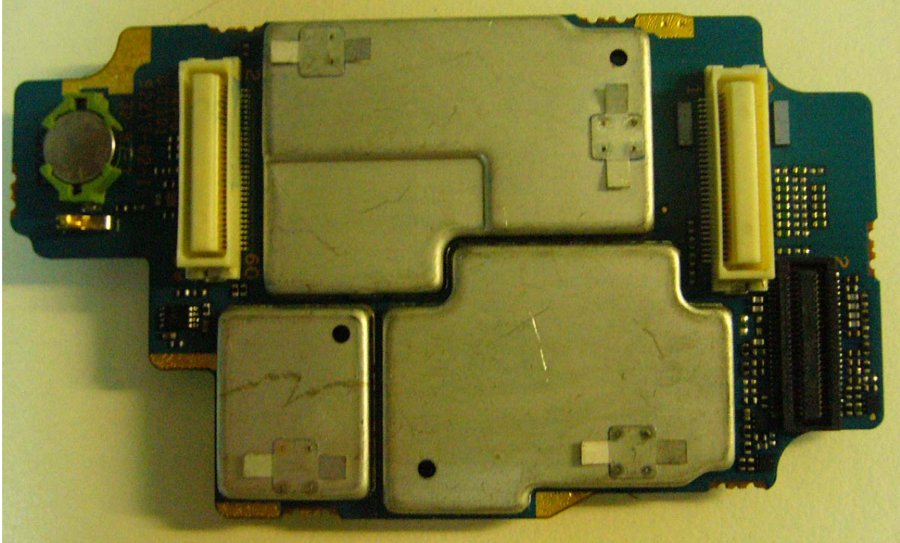
Vocon board with Shields (Top)
