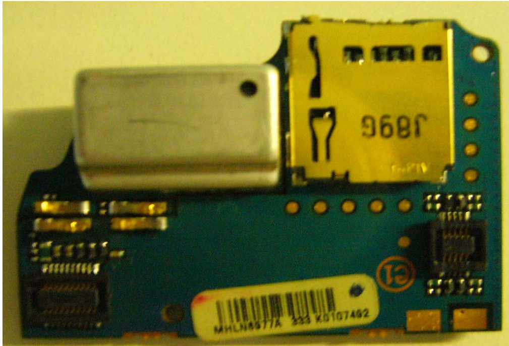
Expander board with shields board (Bottom)
