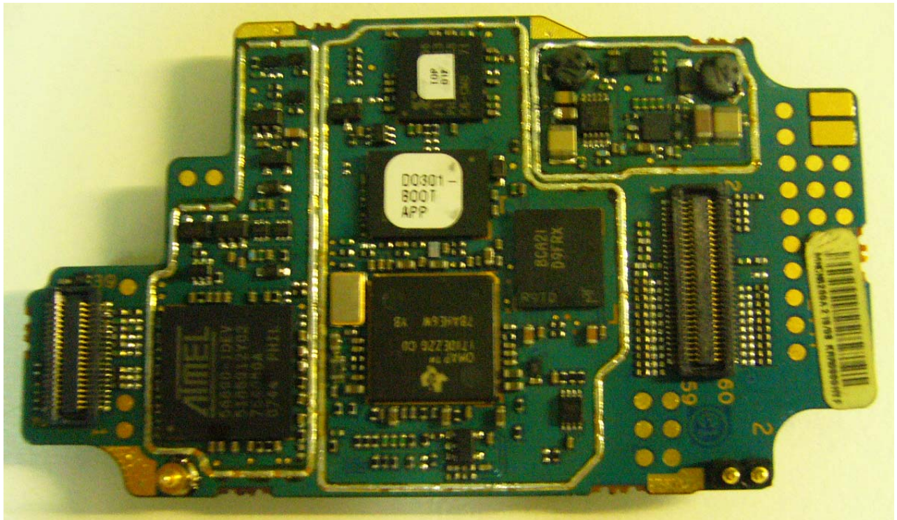
Vocon board without shields board (Bottom)
