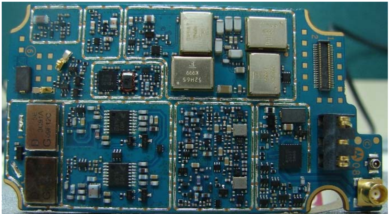
RF board without Shields (Top)
