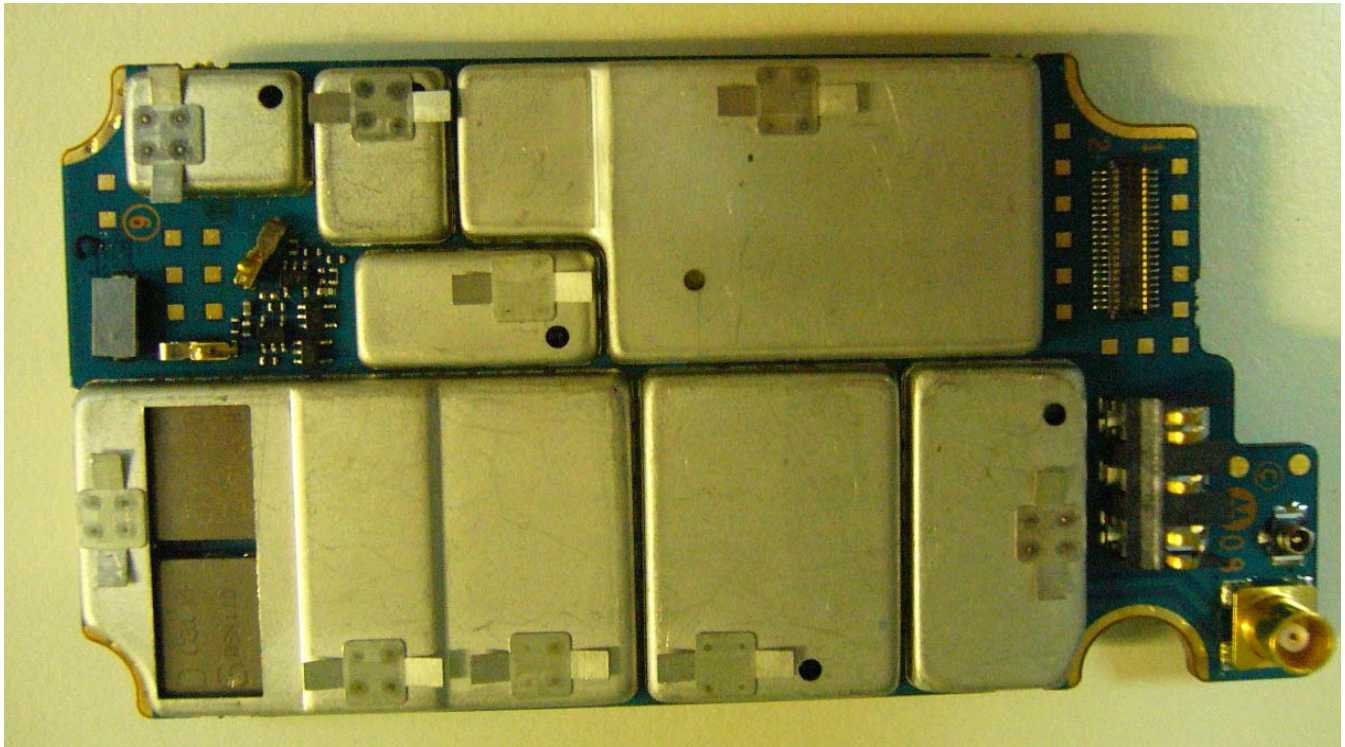
RF board with Shields (Top)
