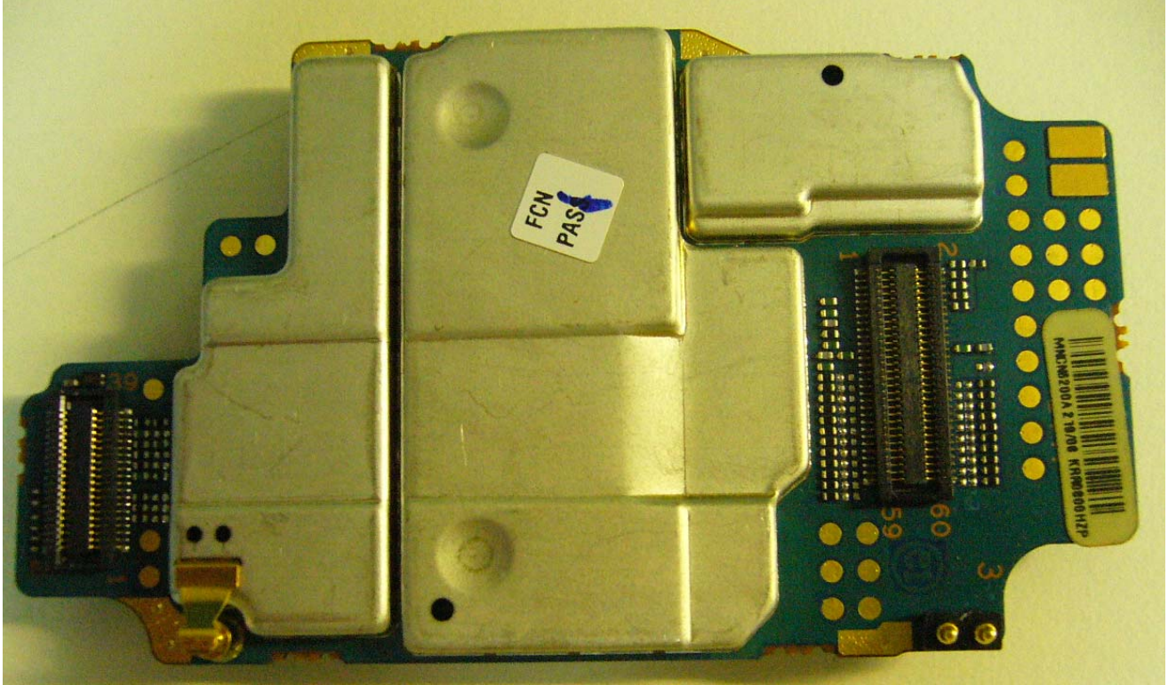
Vocon board with shields board (Bottom)
