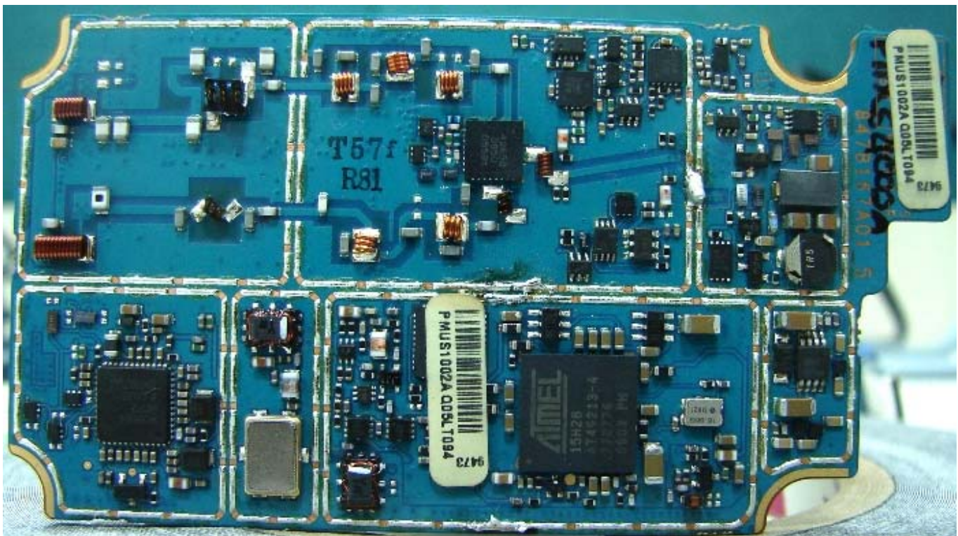
RF board without Shields (Bottom)
