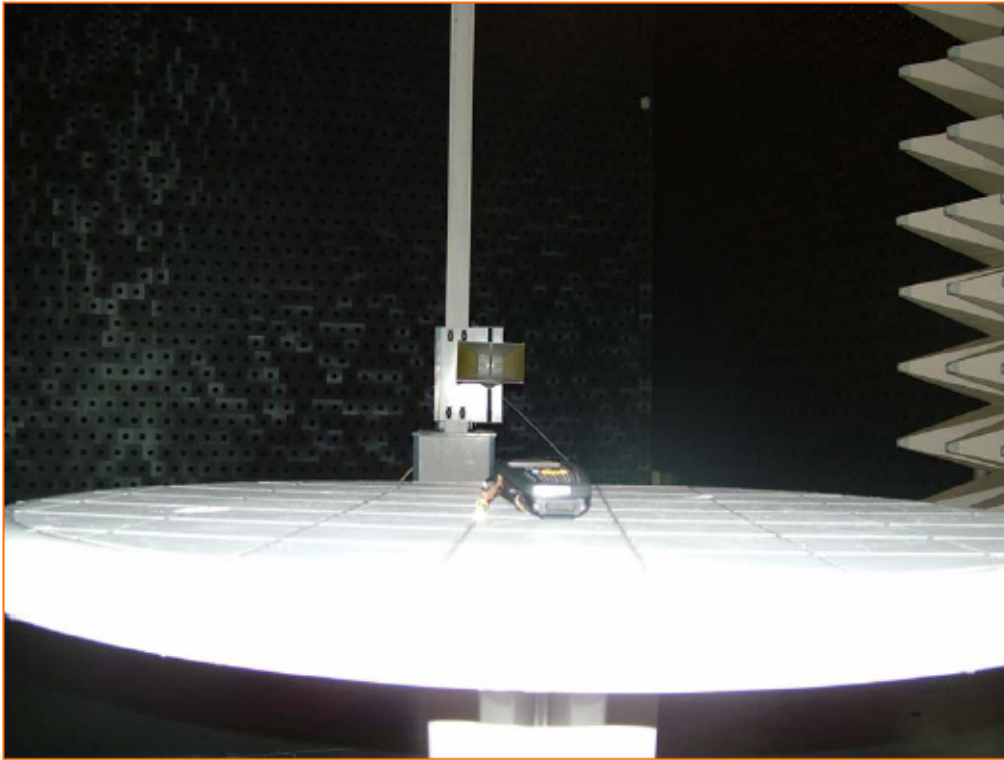
Photograph 4: Radiated measurements
