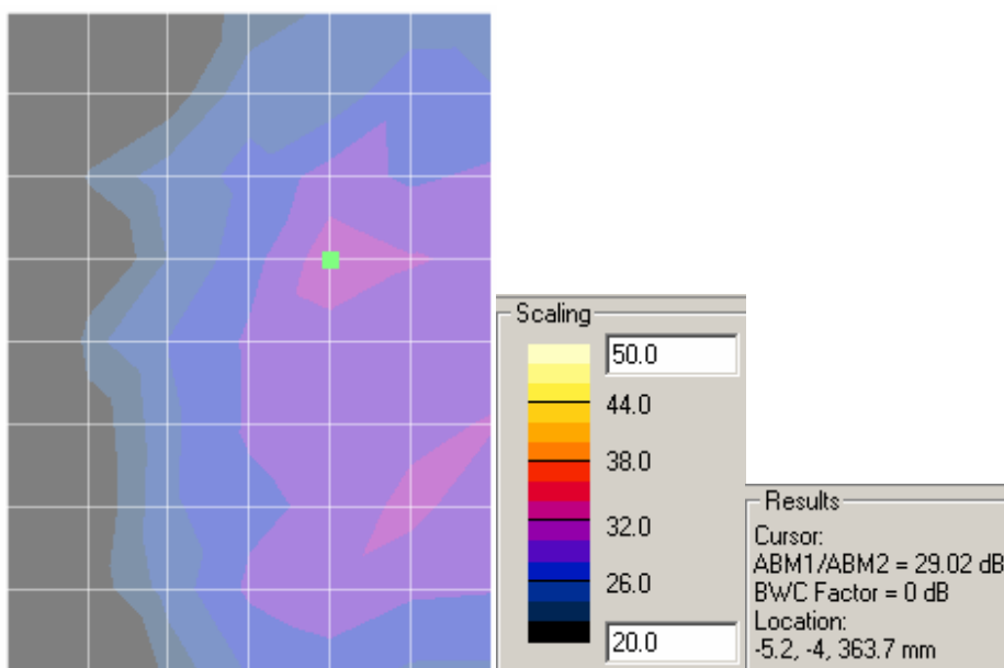
Radial 1 – SNR
