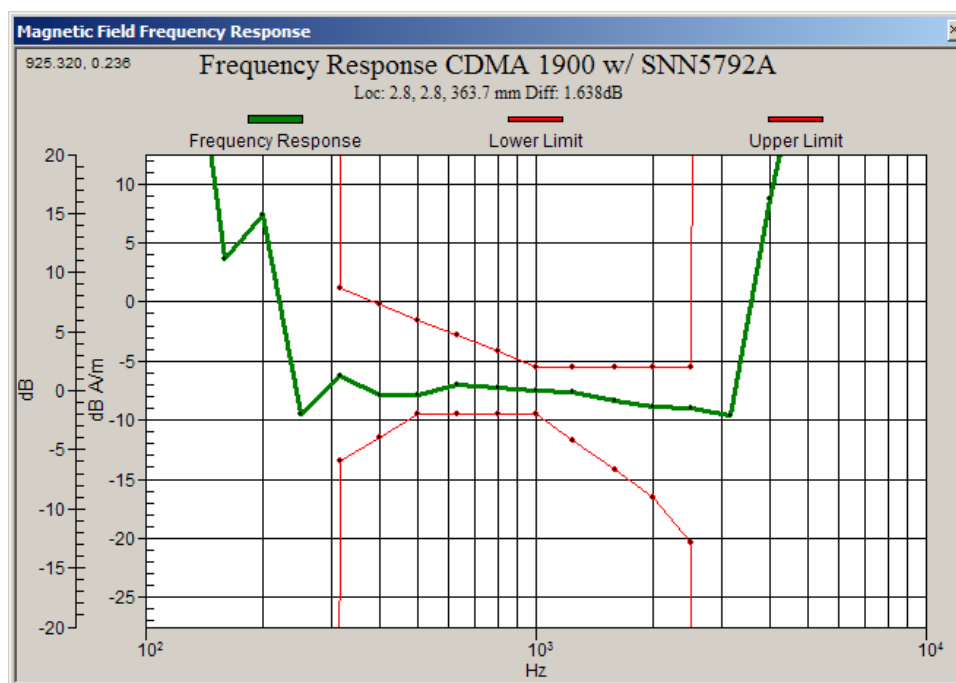
Graph 2: CDMA 1900 Frequency Response
