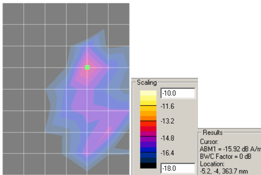
Radial 1 – ABM1
