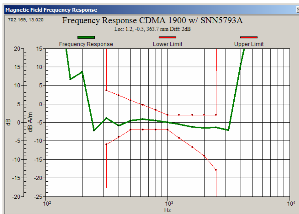
Graph 3: CDMA 1900 Frequency Response with Battery 2
