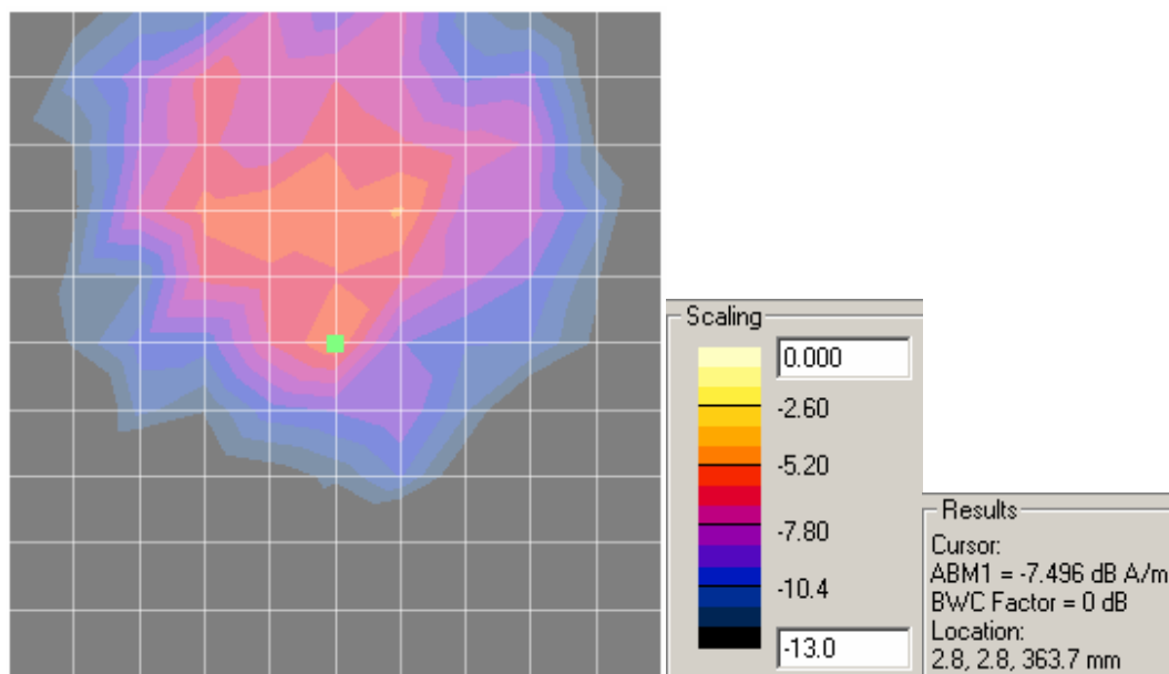
Axial – ABM1
