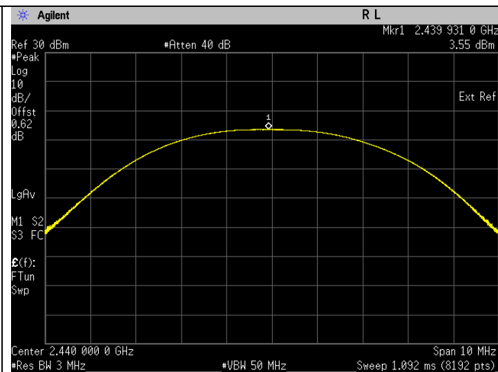
Frequency 2440 MHz
