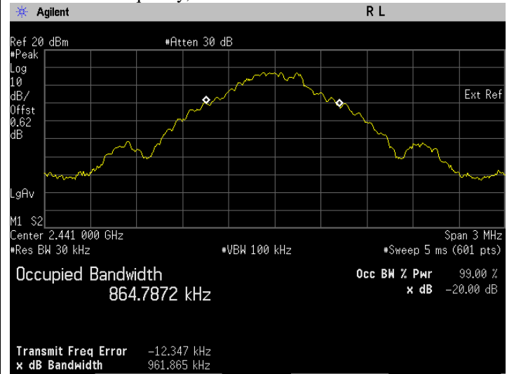
ii. The 20 dB BW & occupied bandwidth test with result at mid frequency, GFSK.
