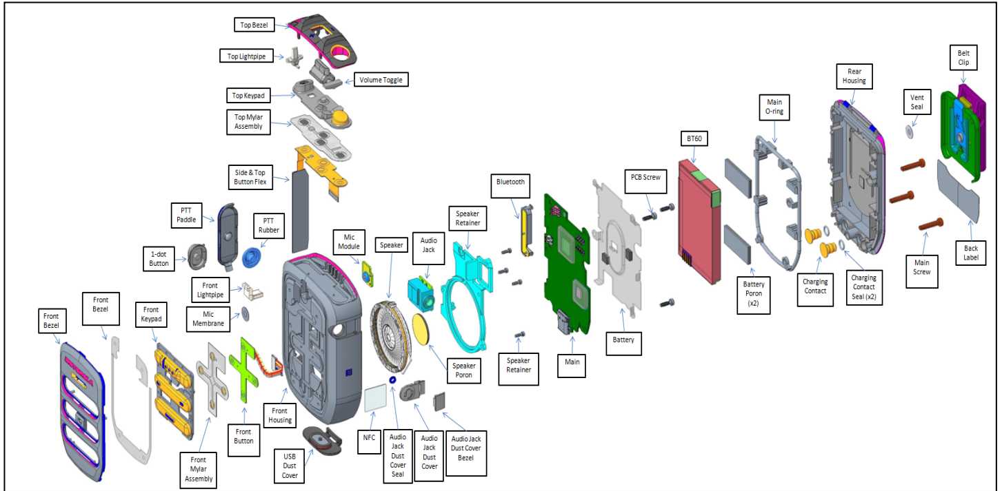
Exploded View
