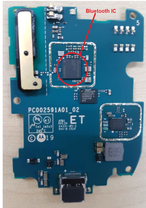
PCB Top without Shield
