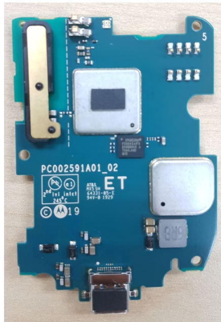
PCB Top with shield
