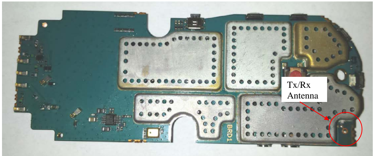
RF board with Shields (Top), (DLR1020, DLR1060)
