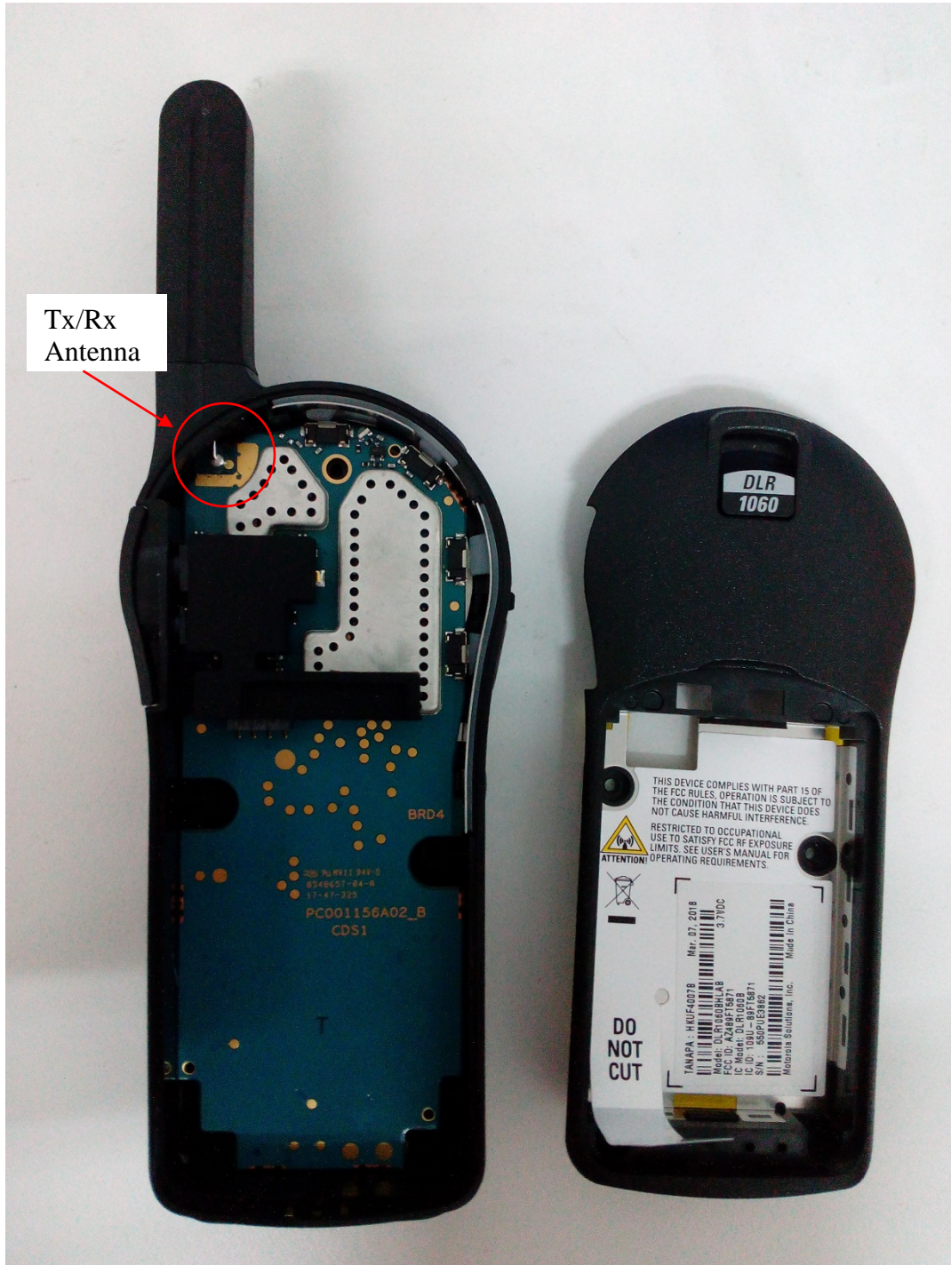
RF board with housing (Back side), (DLR1060) (DLR1060BHLLAA, DLR1060BHLAB)
