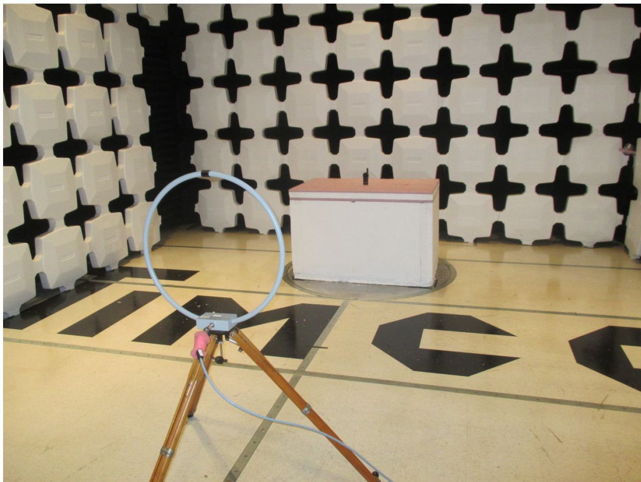
TEST SET UP – RADIATED EMISSIONS – BELOW 30 MHz
