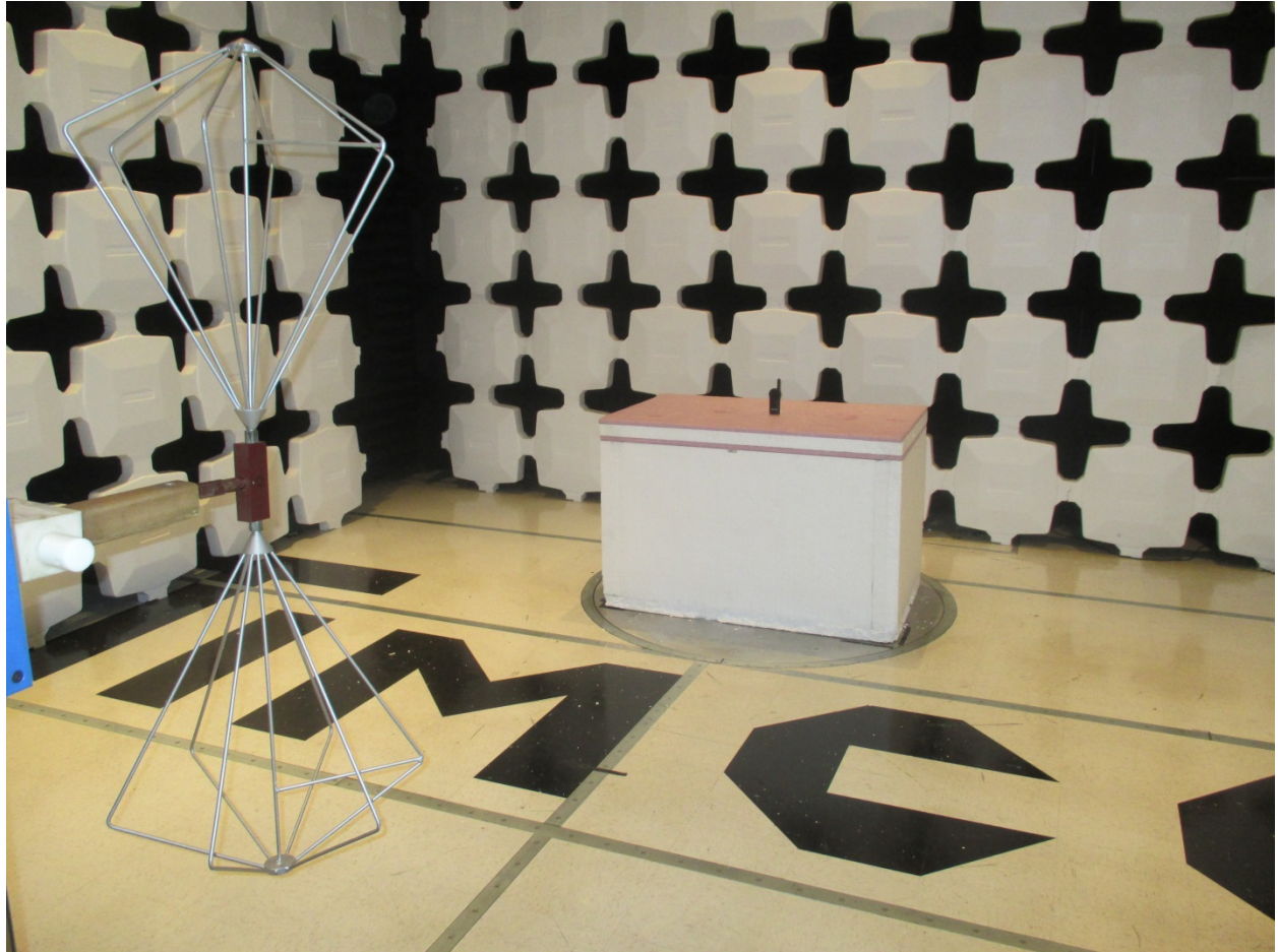
TEST SET UP – RADIATED EMISSIONS ABOVE 30 MHz
