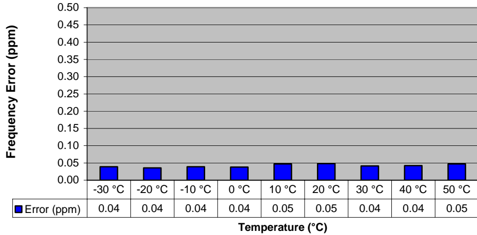
Figure 6-34: Transmitter Frequency Stability (900 MHz band) – Frequency Error vs. Temperature
