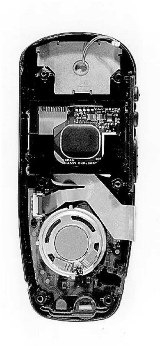
Photograph 9-3: Radio rear housing and main board removed, exposing inside of front housing, and back side of display module and keypad board with speaker.
