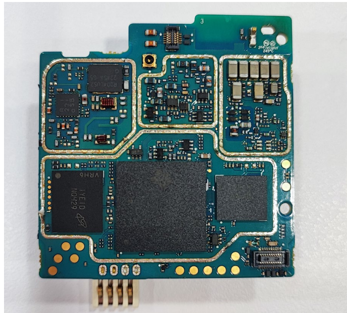
RF board without Shields (Top) - Plain Model
