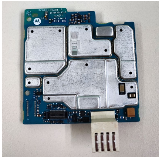
RF board with Shields (Bottom) - Plain Model
