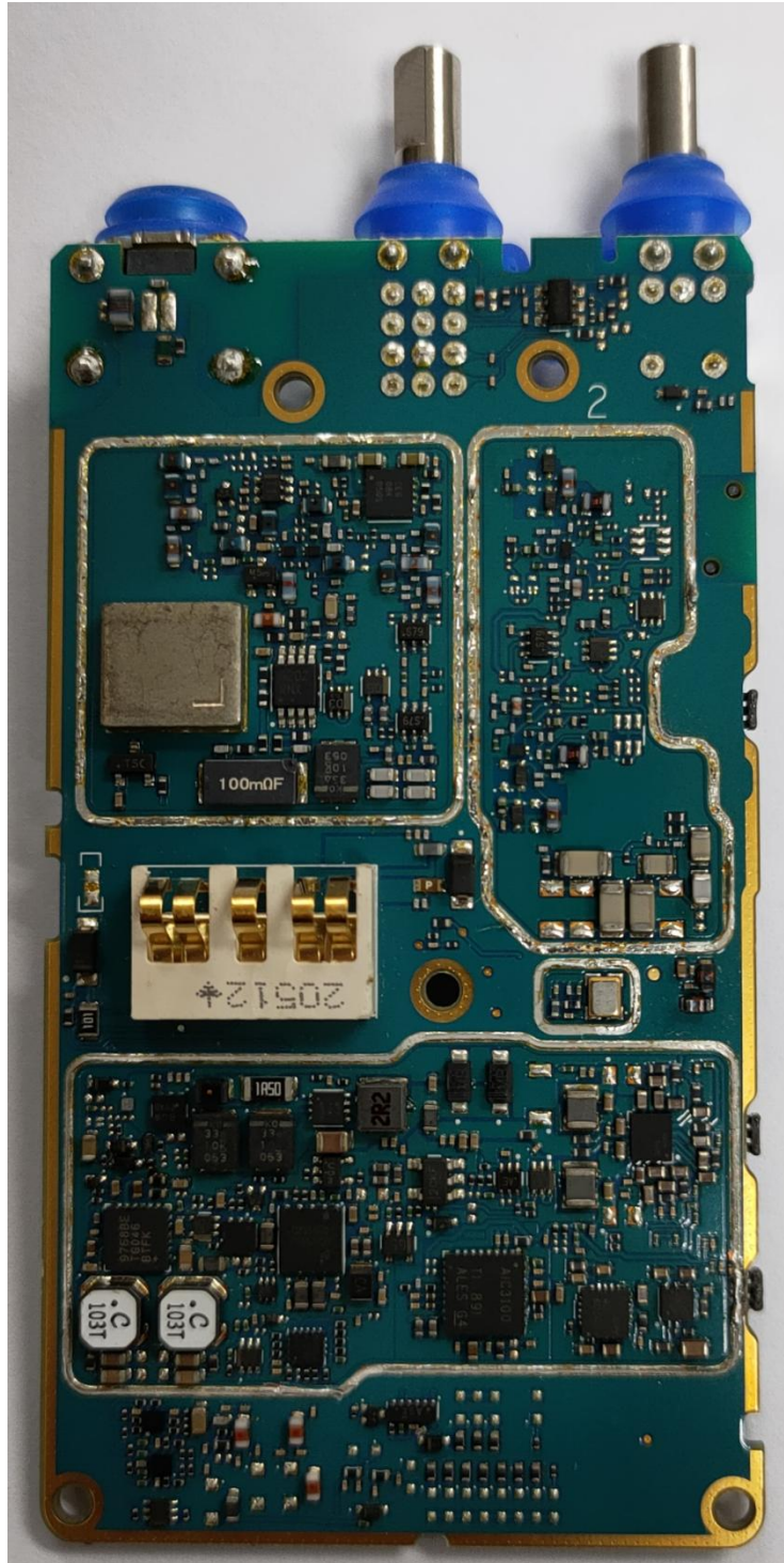
RF board without Shields (Bottom) TIA4950
