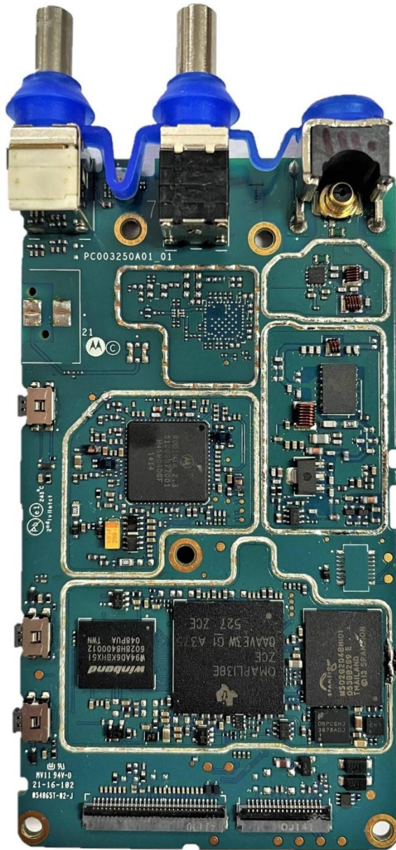
RF board without Shields (Top) TIA4950
