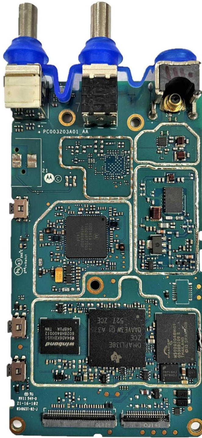
RF board without Shields (Top) Non-TIA4950
