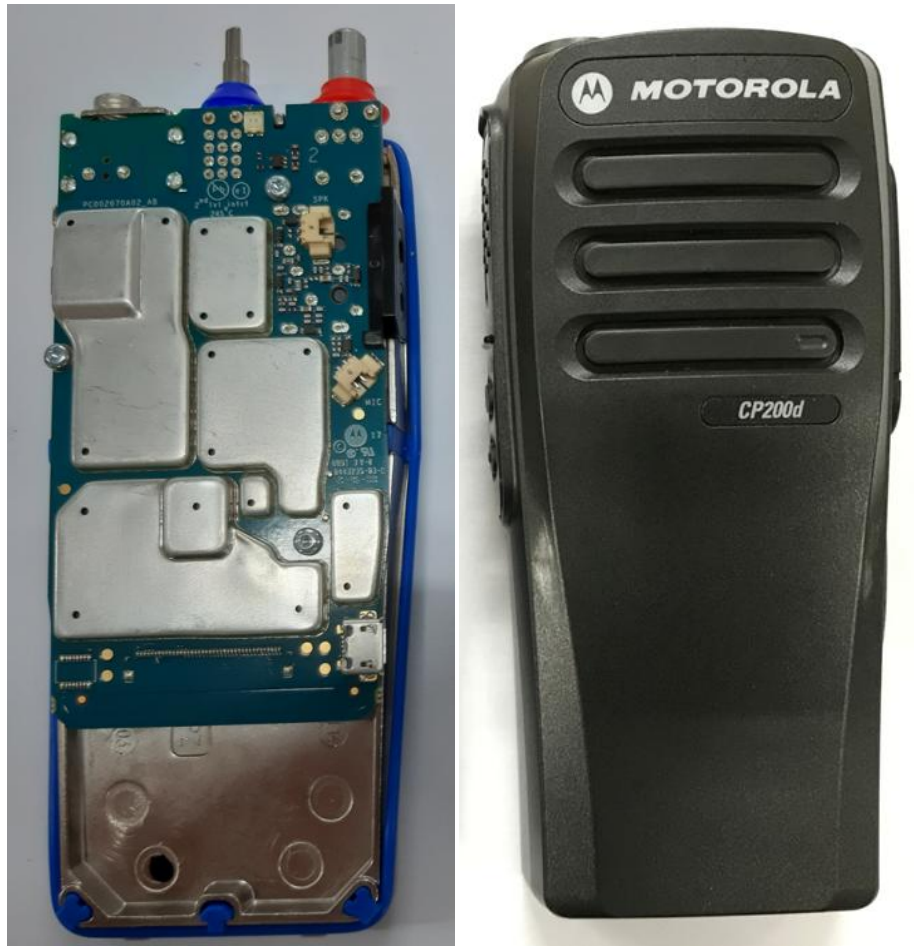
Exhibit 9E - RF board with chassis and housing (front side)
