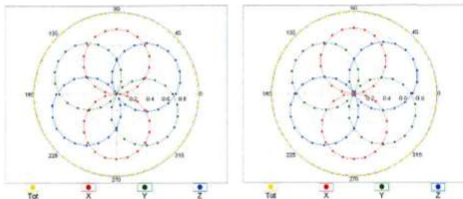
f=600 MHz,TEM
