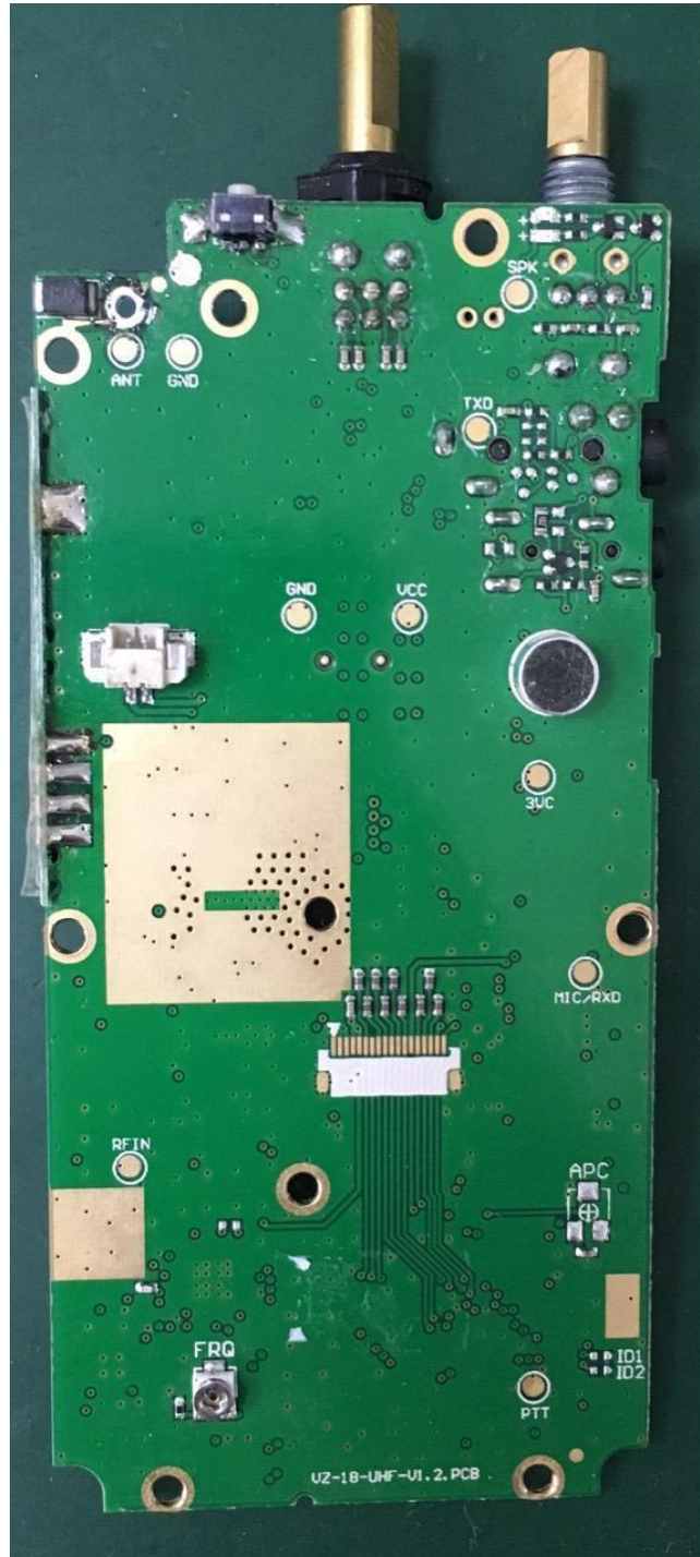
RF Board (Top)
