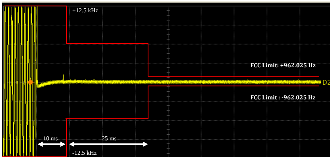
Figure 6I-1: TX 481.0125 MHz - 12.5 KHz Channel Spacing – Transmitter On
