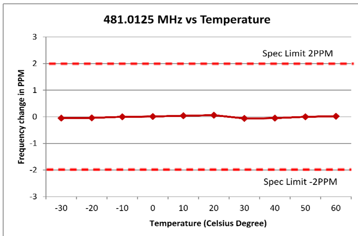
Figure 6H-2: 2.0 ppm Frequency Stability vs. Temperature
