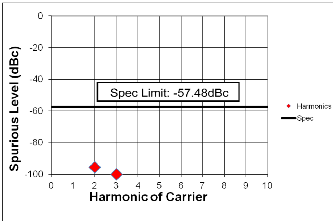
Figure 6G-1: 5.60W 450.0125 MHz, 12.5 kHz Channel Spacing
