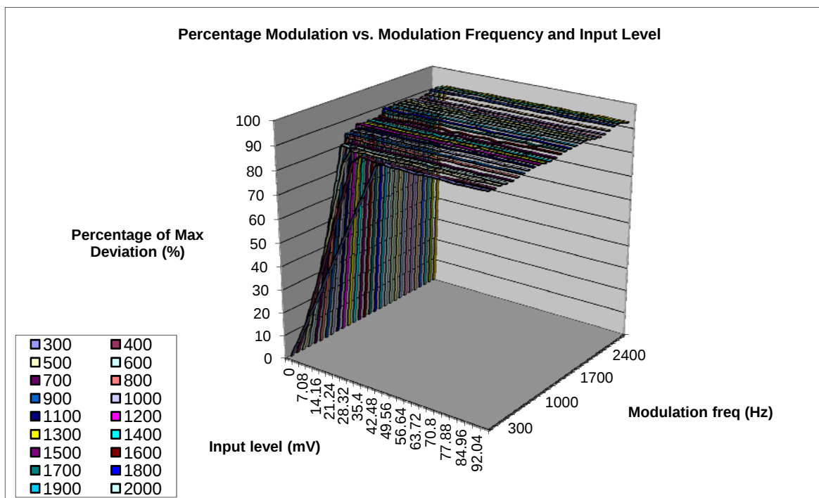
Figure 6D-1: 12.5 kHz Channel Spacing, 481.0125 MHz, Modulation Limiting
