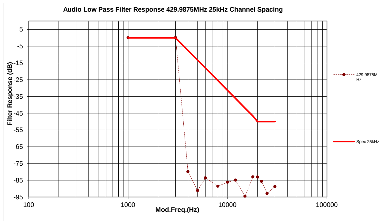
Figure 6C-2: 25 kHz Channel Spacing, 429.9875 MHz, Transmit Audio Low Pass Filter Response (Not for FCC review)
