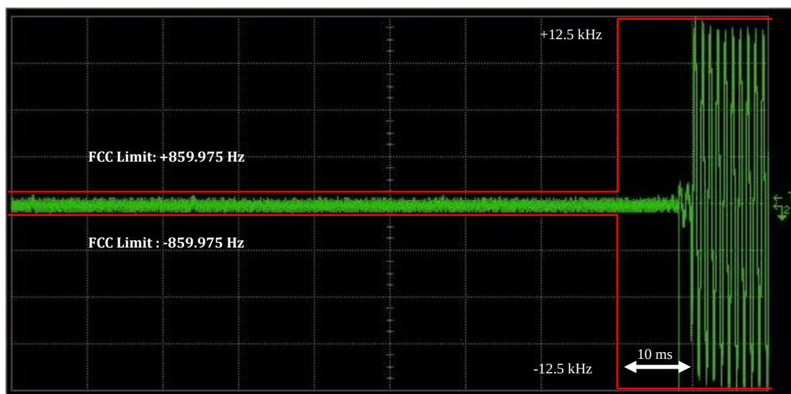
Figure 6I-2: TX 429.9875 MHz - 12.5 KHz Channel Spacing – Transmitter Off
