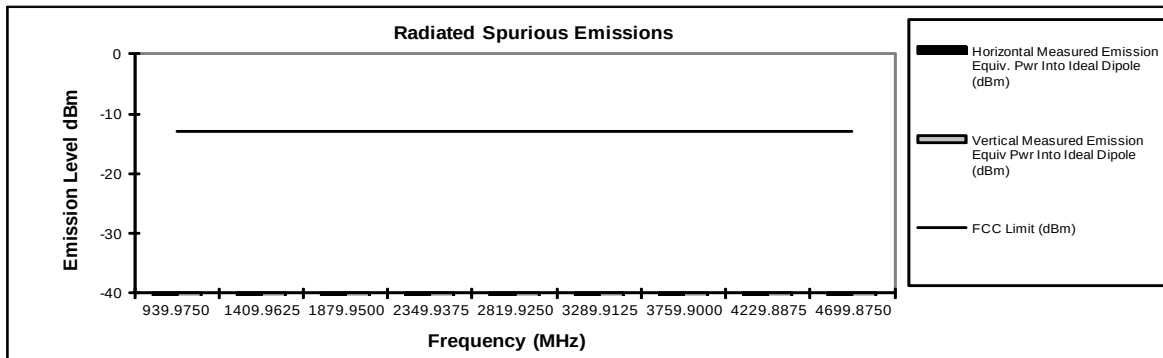
Figure 6F-8: 5.70W 469.9875 MHz, 25 kHz Channel Spacing (Not for FCC Review)
