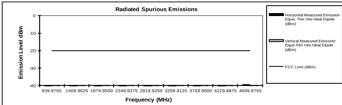
Figure 6F-4: 5.70W 469.9875 MHz, 12.5 kHz Channel Spacing
