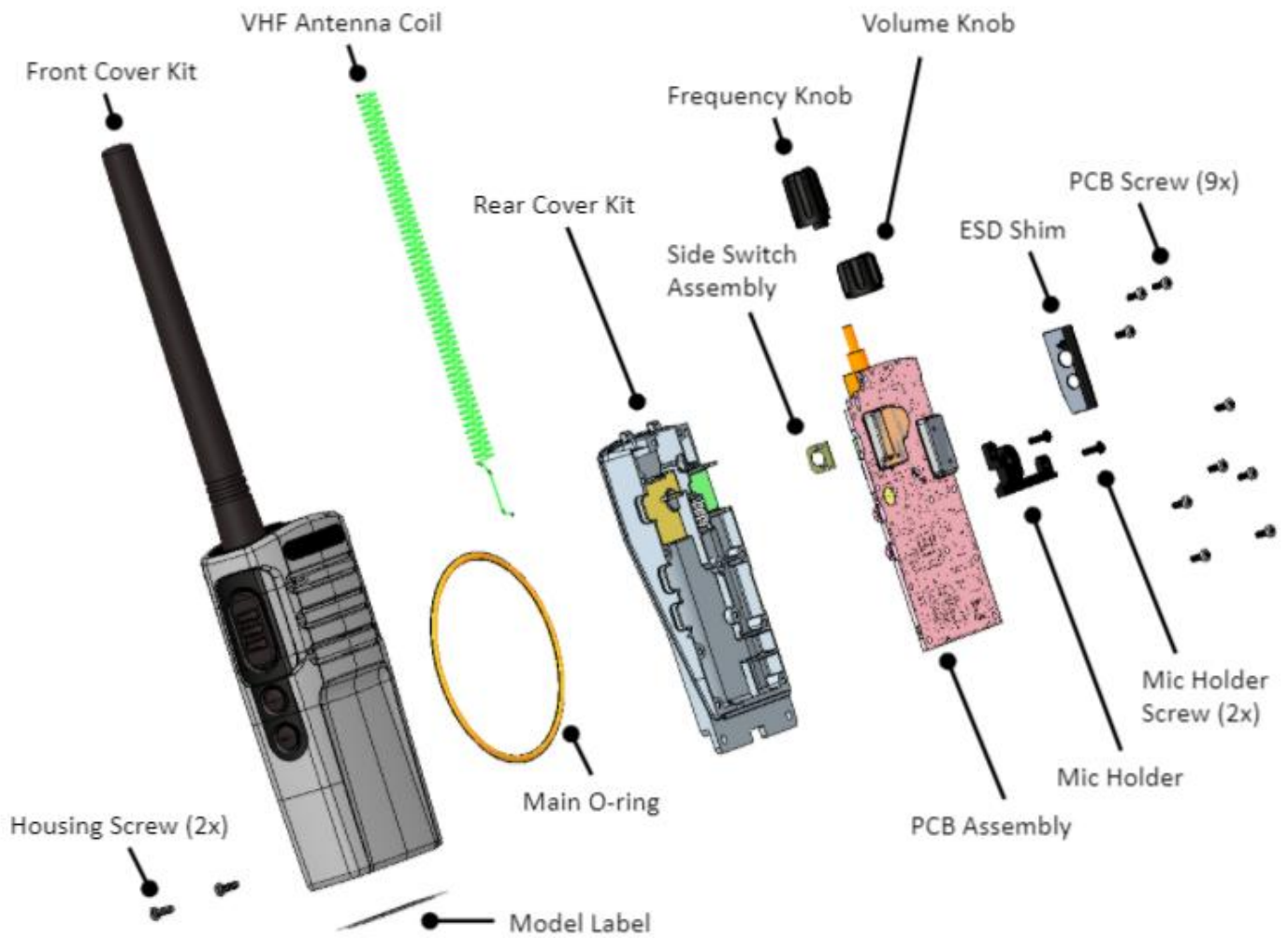
Exploded View of Radio
