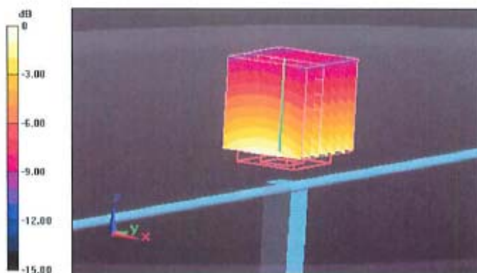
0 dB = 1.890mW/g
