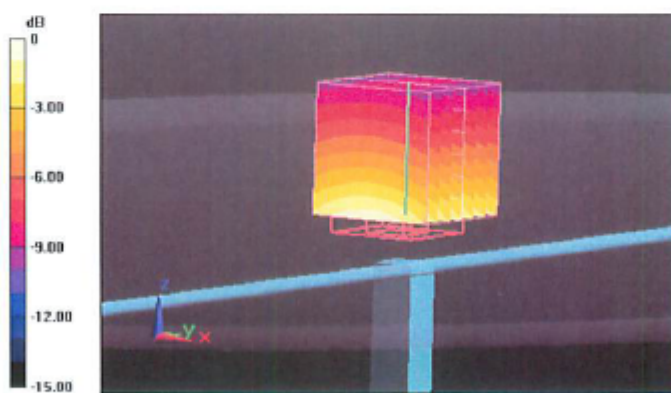
0 dB = 1.940mW/g
