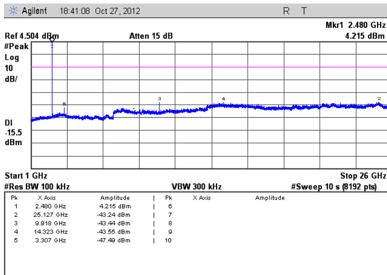
Figure 7.5.3.2-18: 1 GHz – 26 GHz – High Channel (8DPSK)
