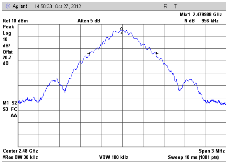
Figure 7.4.4.2-3: 20dB BW High Channel (GFSK)
