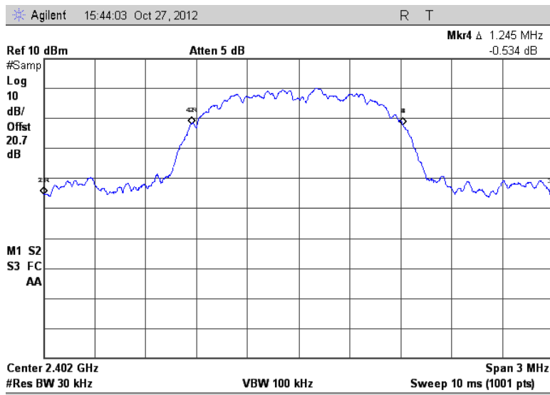
Figure 7.4.4.2-16: 99% OBW Low Channel (8DPSK)
