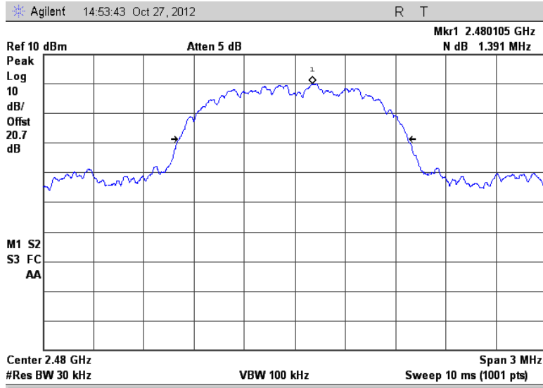
Figure 7.4.4.2-15: 20dB BW High Channel (8DPSK)
