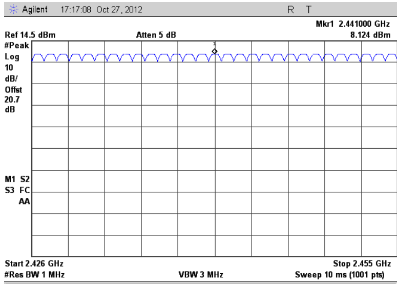
Figure 7.4.2.2-2: Number of Hopping Channels (26 – 54)
