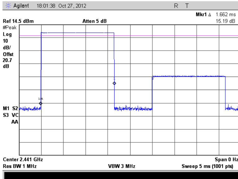
Figure 7.4.3.2-2: Channel Dwell Time – DH3
