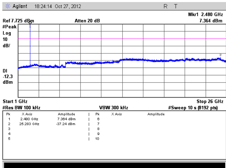
Figure 7.5.3.2-6: 1 GHz – 26 GHz – High Channel (GFSK)
