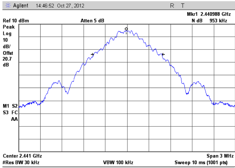
Figure 7.4.4.2-2: 20dB BW Middle Channel (GFSK)
