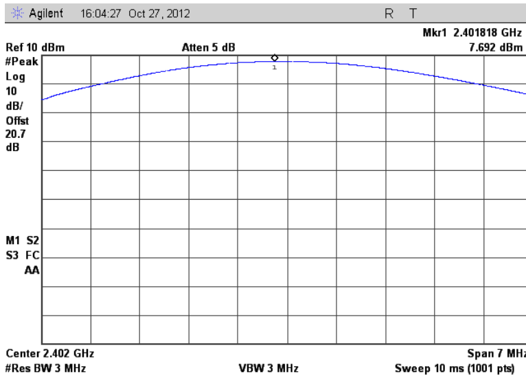
Figure 7.3.2-4: RF Output Power ( \pi/4 DQPSK) - Low Channel
