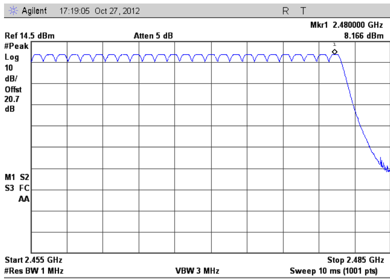
Figure 7.4.2.2-3: Number of Hopping Channels (55 – 79)
