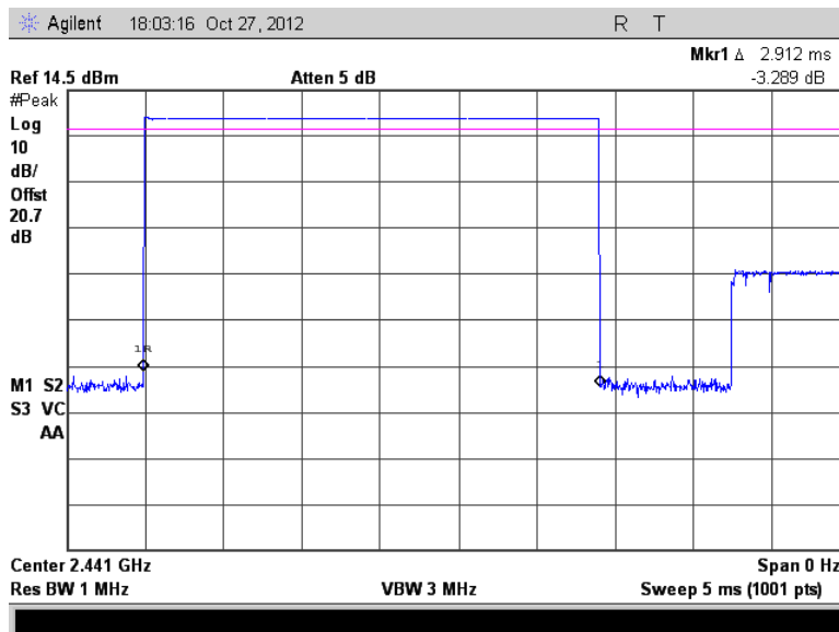
Figure 7.4.3.2-3: Channel Dwell Time – DH5
