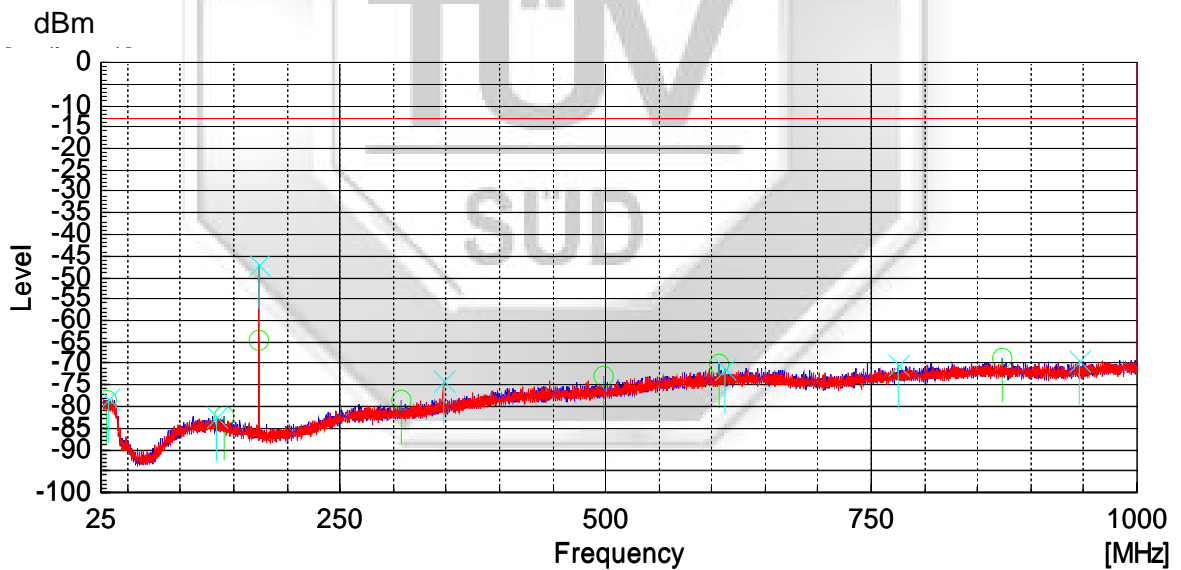
173.3875MHz (Analog) 25MHz – 1GHz
