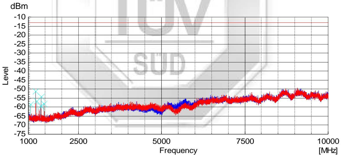
161.7MHz (Analog) 1GHz – 10GHz
