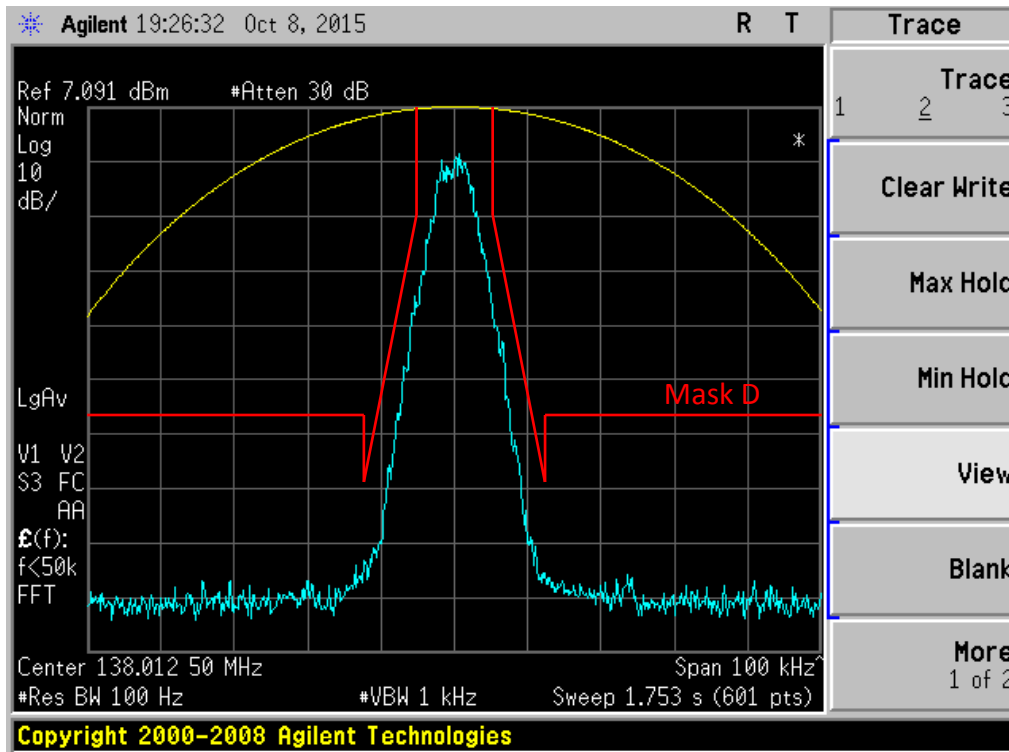
Figure 6E-8: 138.0125 MHz, O.153 Test Pattern 4FSK Voice Modulation Only, 7K60F1E Mask D (Not applicable for FCC)
