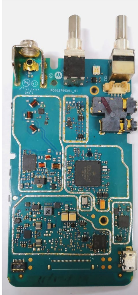
RF board without Shields (Top) -Non Keypad (NKP) model, AAH87JDC9JA2AN-
