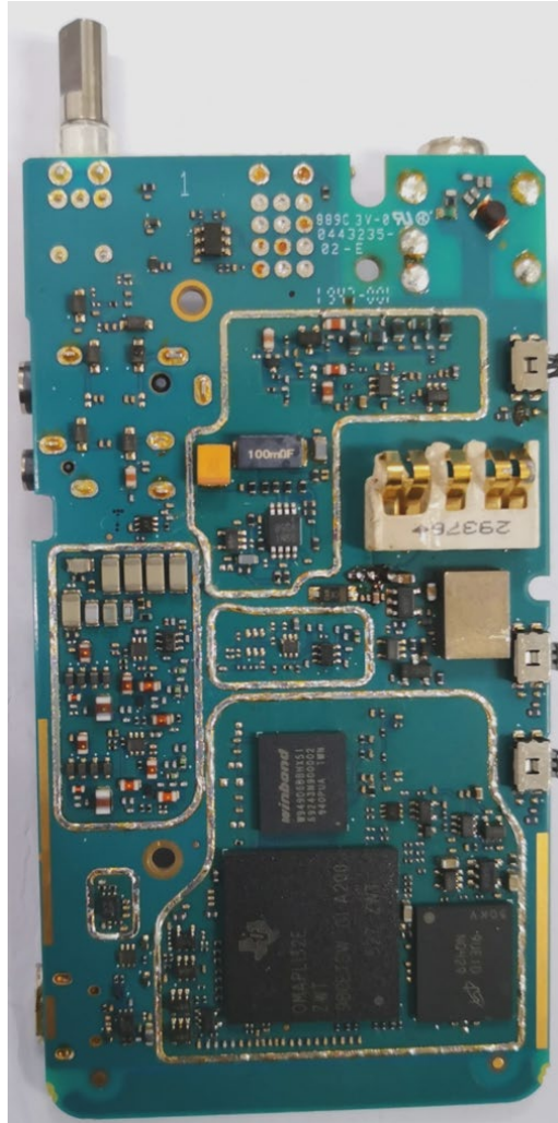
RF board without Shields (Bottom) -Full Keypad (FKP) model, AAH87JDF9JA2AN-
