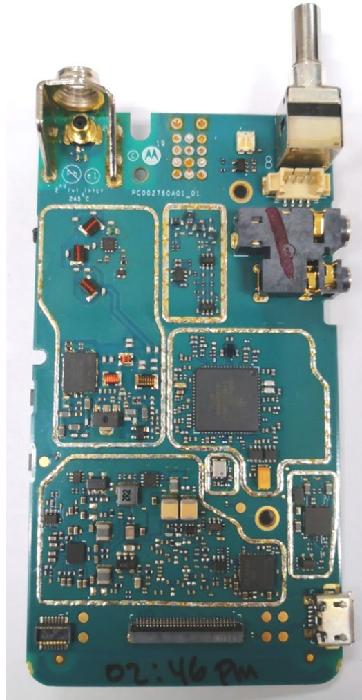
RF board without Shields (Top) -Full Keypad (FKP) model, AAH87JDF9JA2AN-
