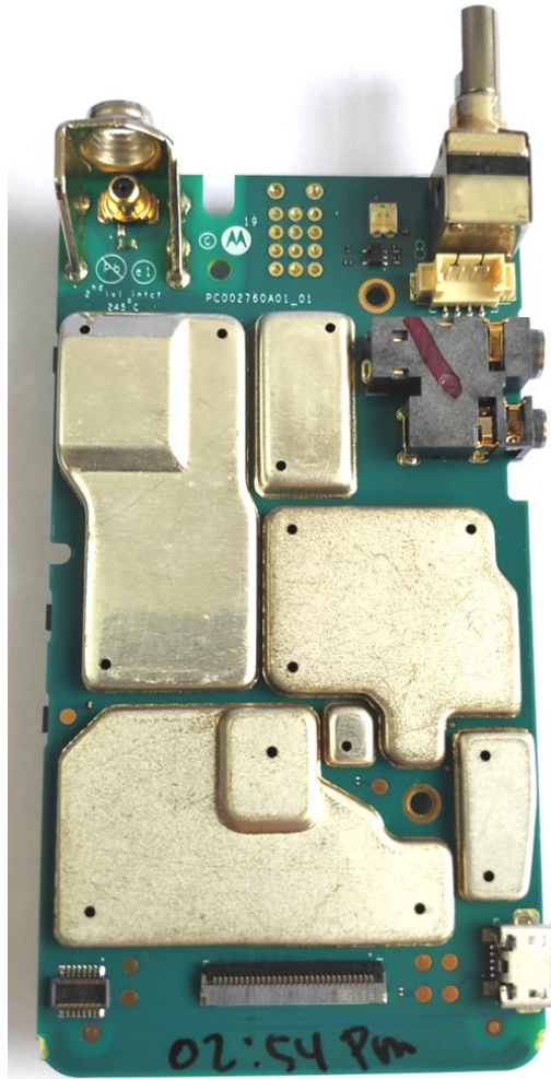
RF board with Shields (Top) -Limited Keypad (LKP) model, AAH87JDH9JA2AN-
