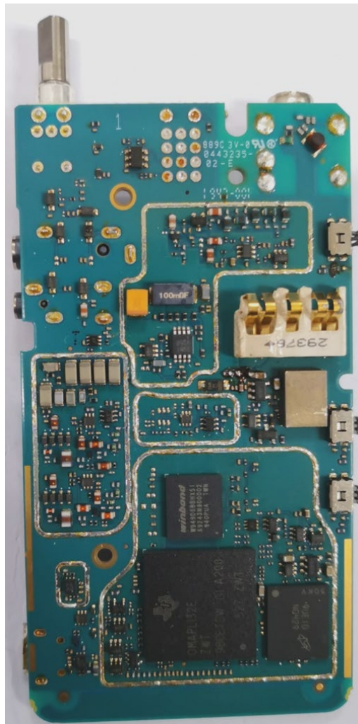
RF board without Shields (Bottom) -Limited Keypad (LKP) model, AAH87JDH9JA2AN-
