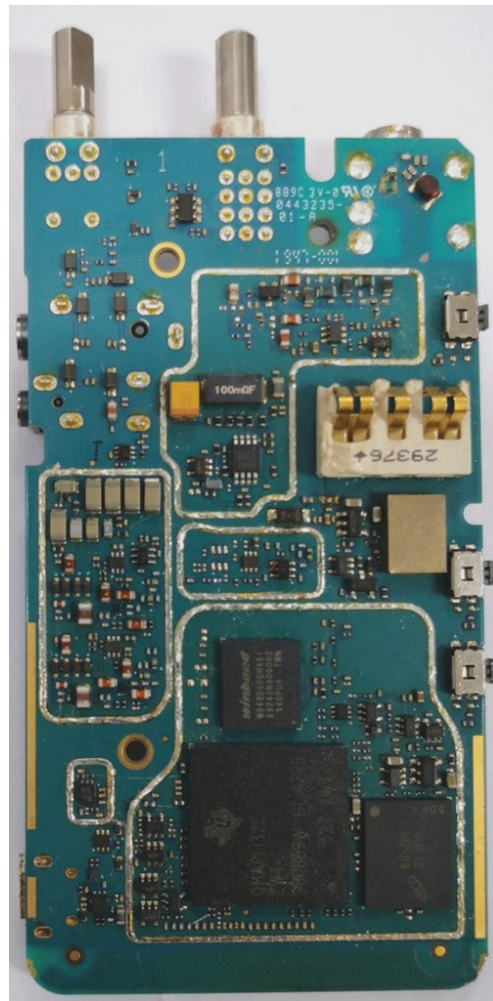
RF board without Shields (Bottom) -Non Keypad(NKP) model, AAH87JDC9JA2AN-
