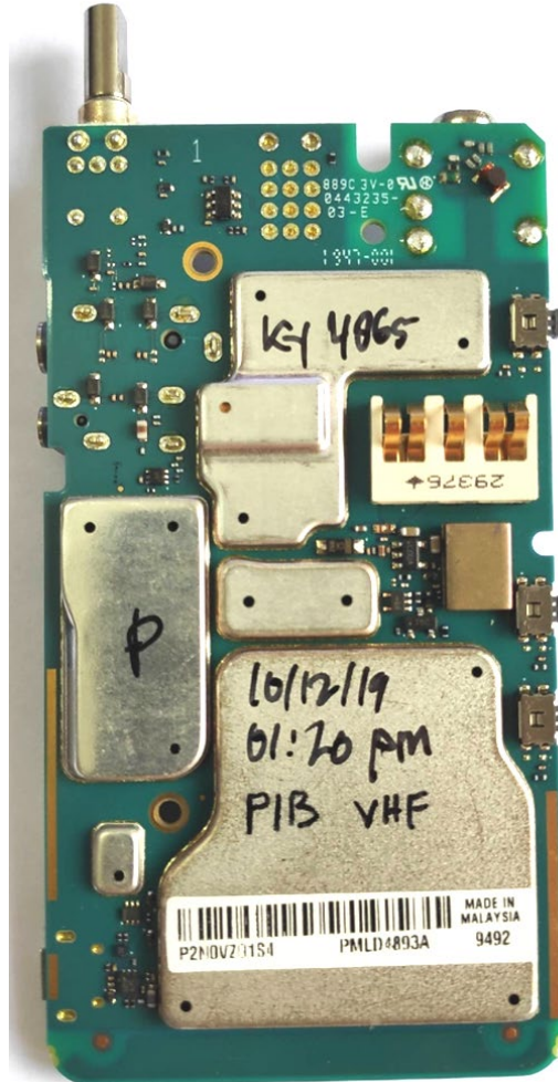
RF board with Shields (Bottom) - Full Keypad (FKP) model, AAH87JDF9JA2AN-
