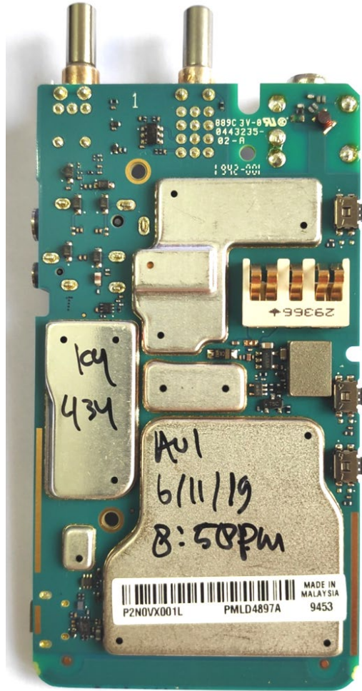
RF board with Shields (Bottom) -Non Keypad (NKP) model, AAH87JDC9JA2AN-
