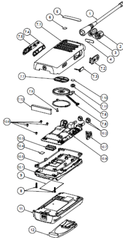
Exploded View of Radio -Non Keypad(NKP) model, AAH87JDC9JA2AN-
