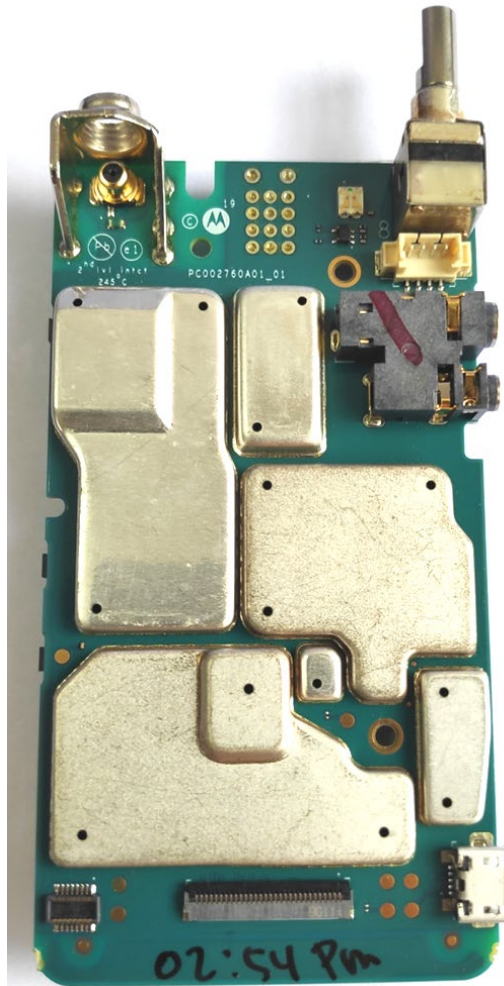
RF board with Shields (Top) -Full Keypad (FKP) model, AAH87JDF9JA2AN-
