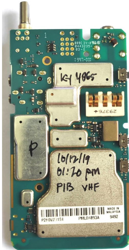
RF board with Shields (Bottom) -Limited Keypad (LKP) model, AAH87JDH9JA2AN-
