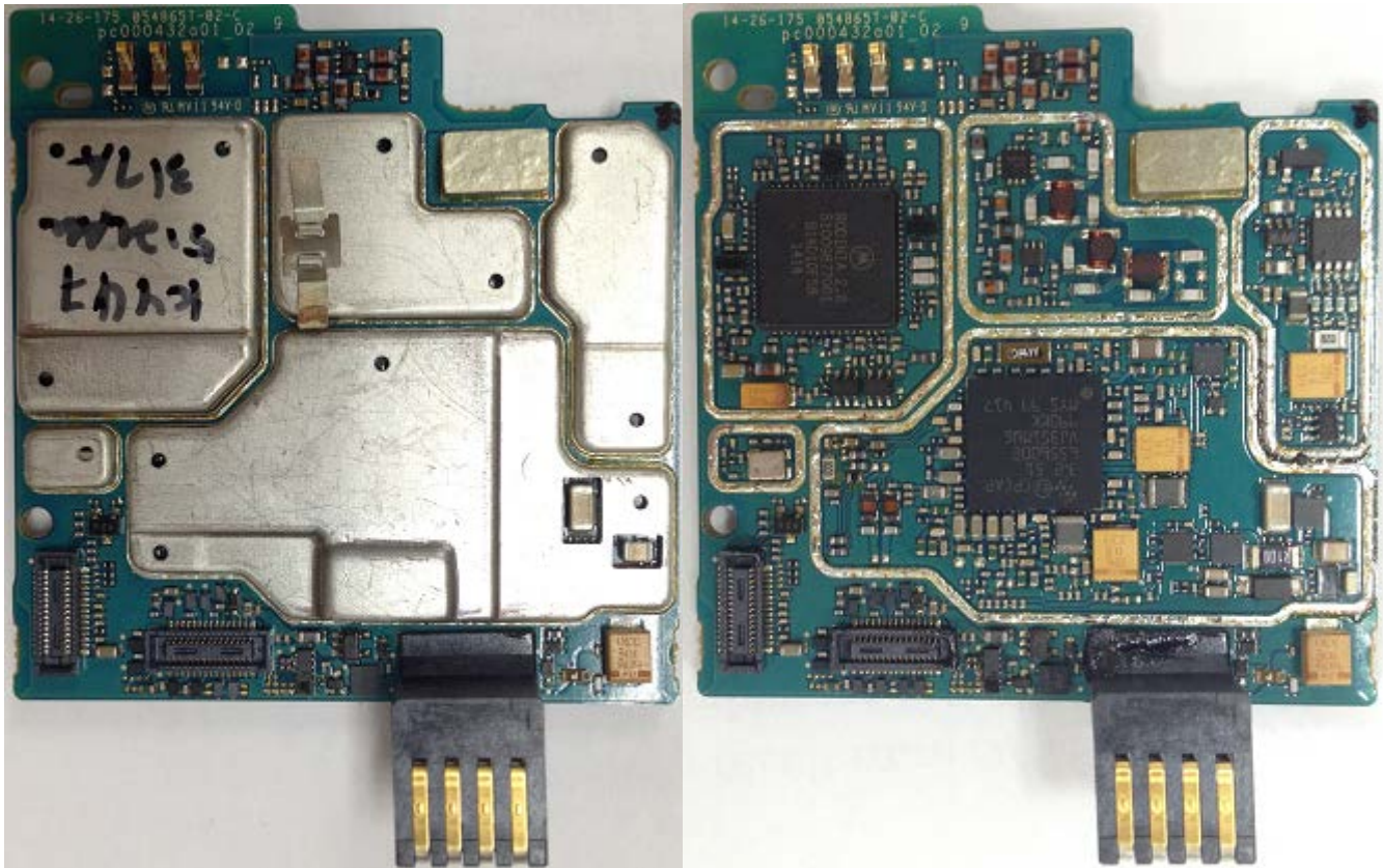
RF board with and without Shields (Top)
