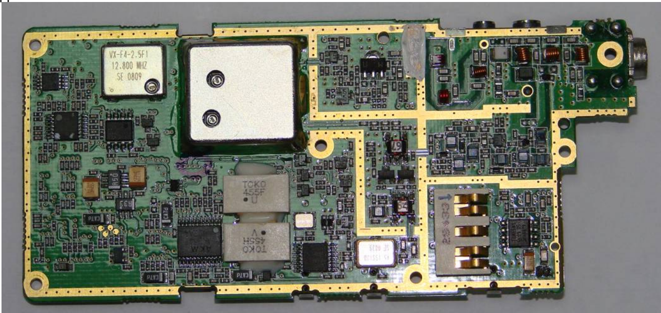
Figure 9-3: Bottom Side of PCB (with shield)
