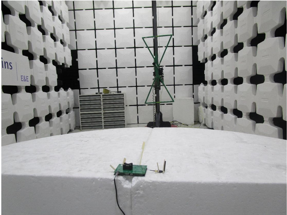
Radiated tests 30MHz to 1GHz
