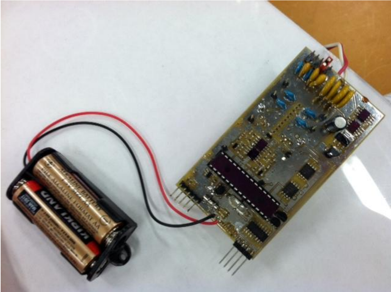
Figure 1 - Internal Photo, Circuit board with RTC backup battery
