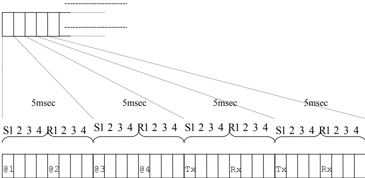
Fig. 1-4 FRAME structure of COMMUNICATION CHANNEL
