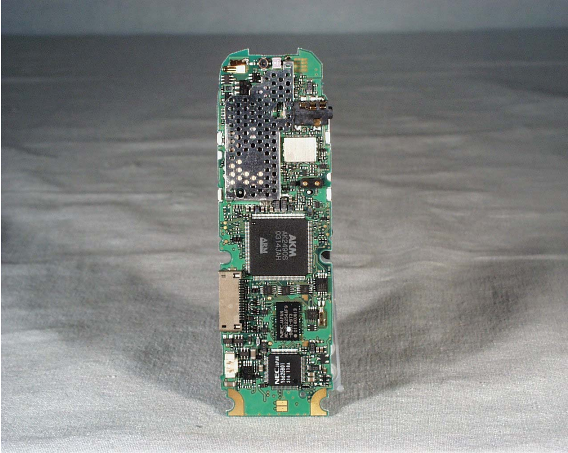
Photograph 2 shows the component side of the PC board.
