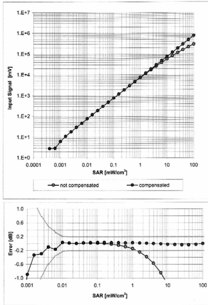
Uncertainty of Linearity Assessment: \pm 0.6\% ( k=2 )
