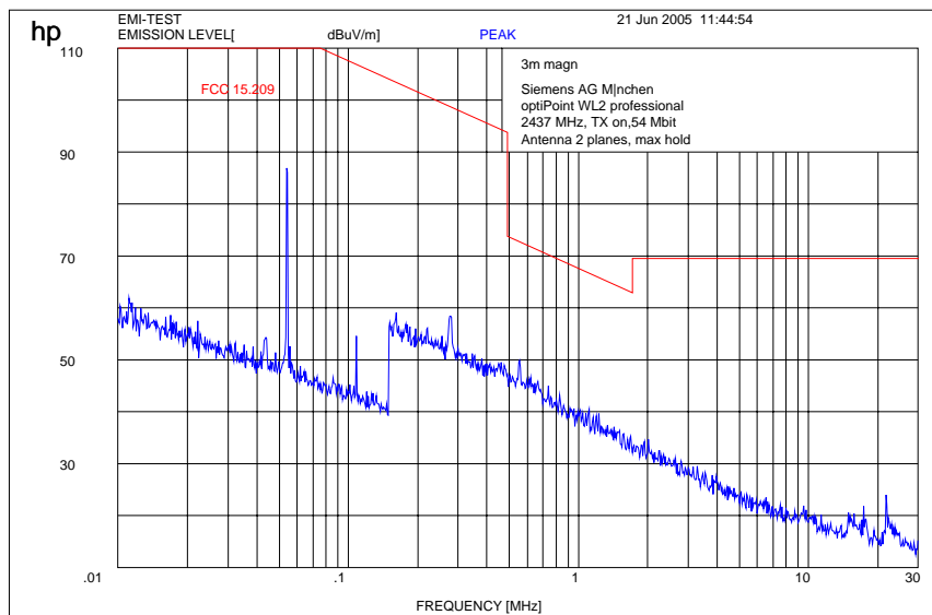
Plot 1: 9 kHz – 30 MHz radiated emissions
