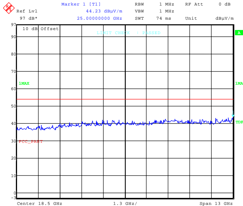
Plot 4: 12-25 GHz (receiver)
