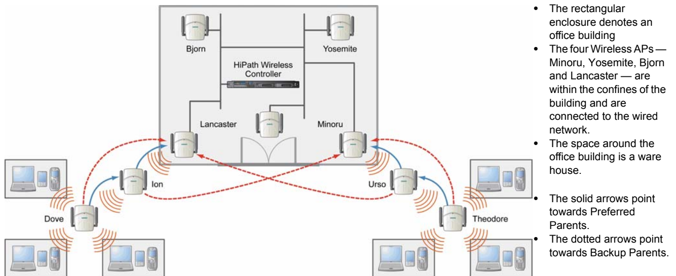
Figure 18 Deployment Example
