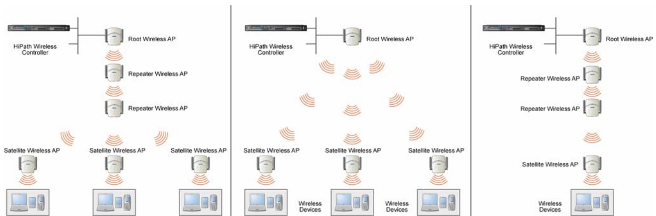
Figure 17 Examples of WDS deployment
