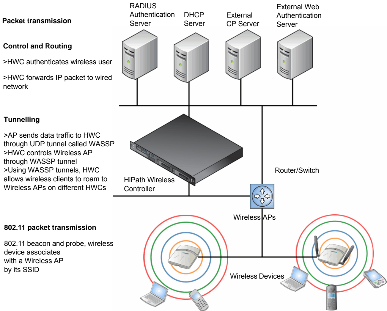
Figure 3 Traffic Flow diagram
