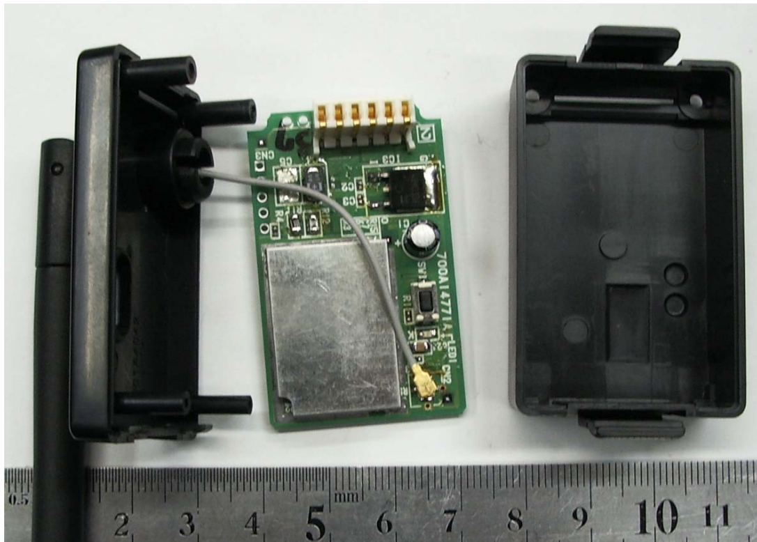
Figure 3 Internal View (Removed Cover)
