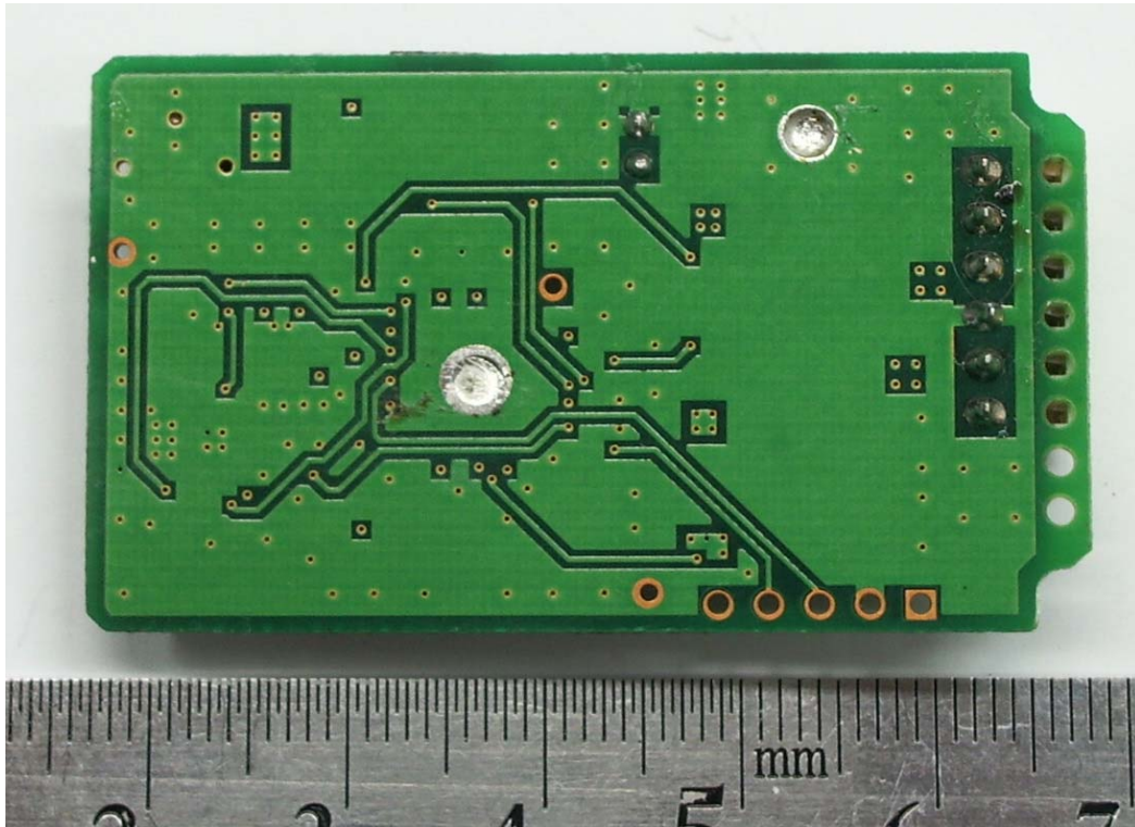
Figure 6 Internal View (Control Board , Back View)
