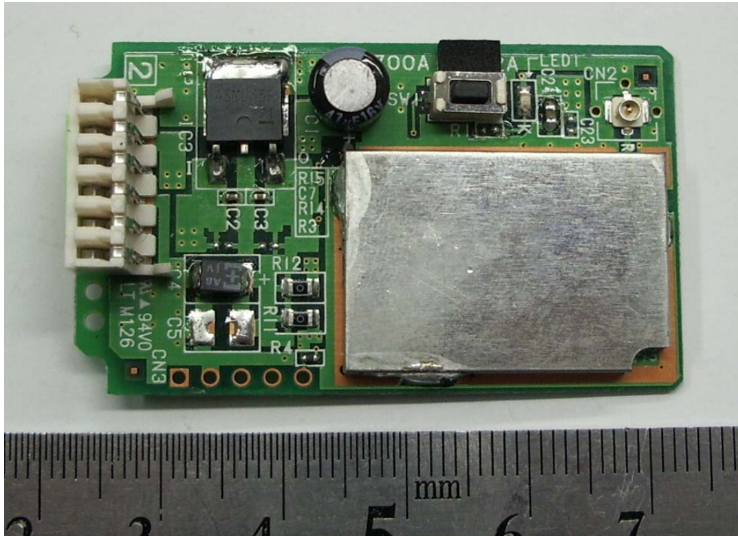
Figure 4 Internal View (Control Board , Front View with Shield)
