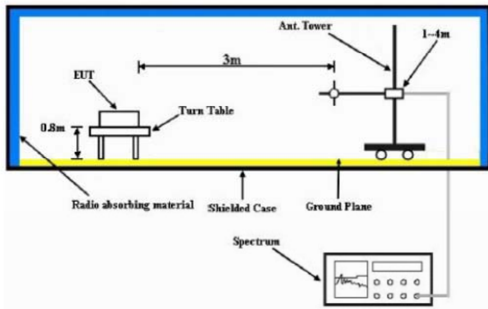
Radiated test setup drawing
