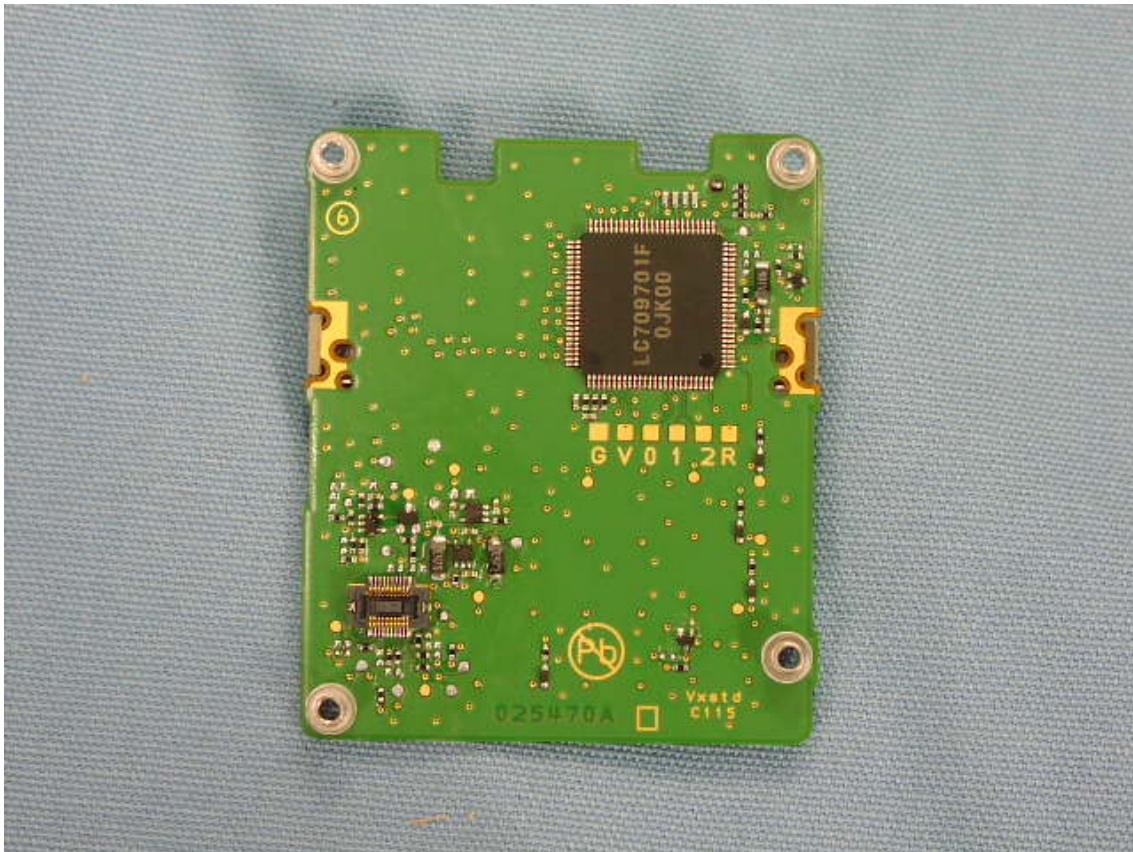
Side B of DISPLAY-UNIT (EVX-534 / EVX-539)
