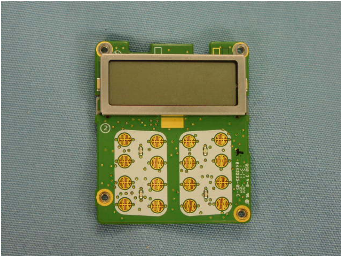
Side A of DISPLAY-UNIT (EVX-534 / EVX-539)
