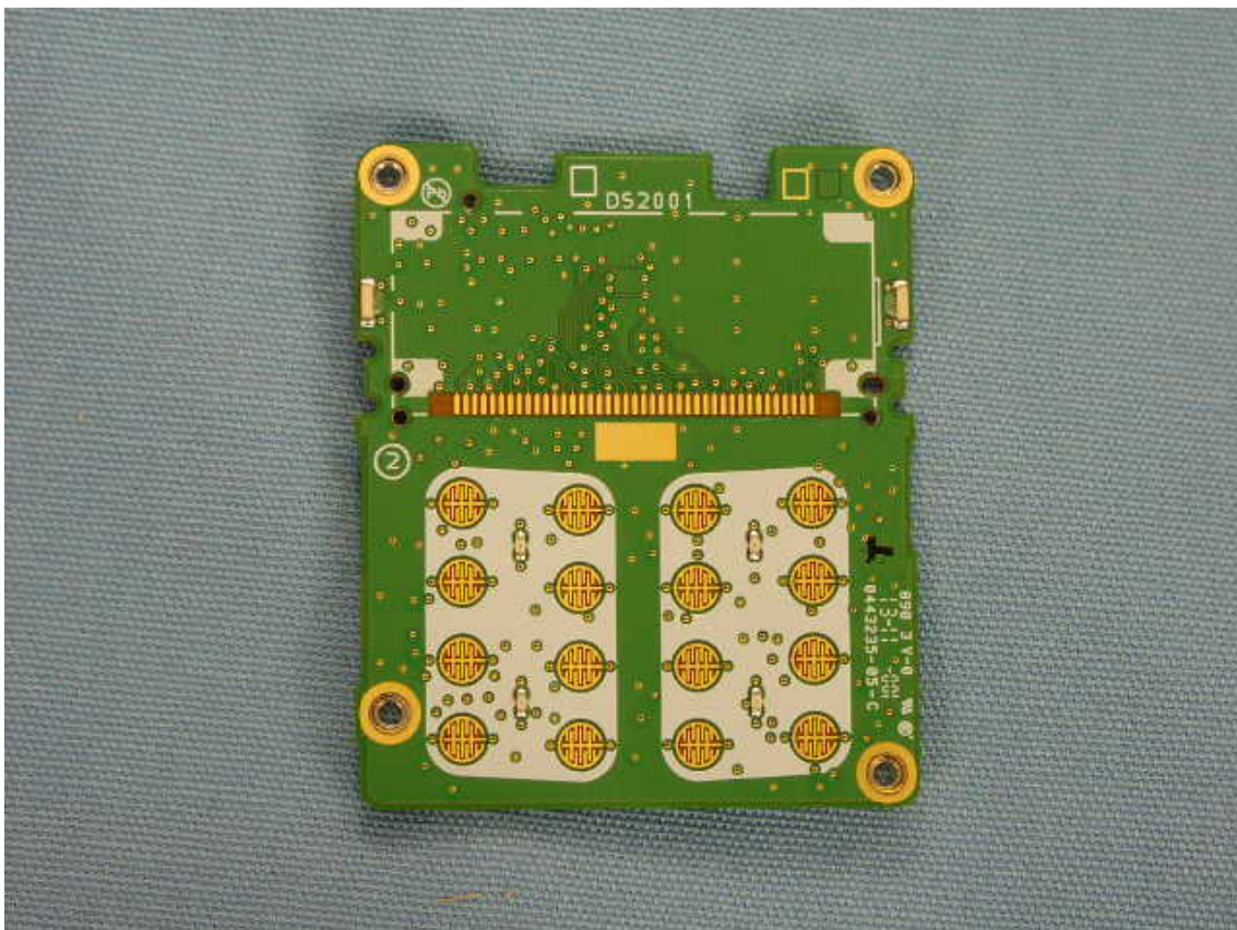
Side A of DISPLAY-UNIT Without LCD-UNIT(EVX-534 / EVX-539)
