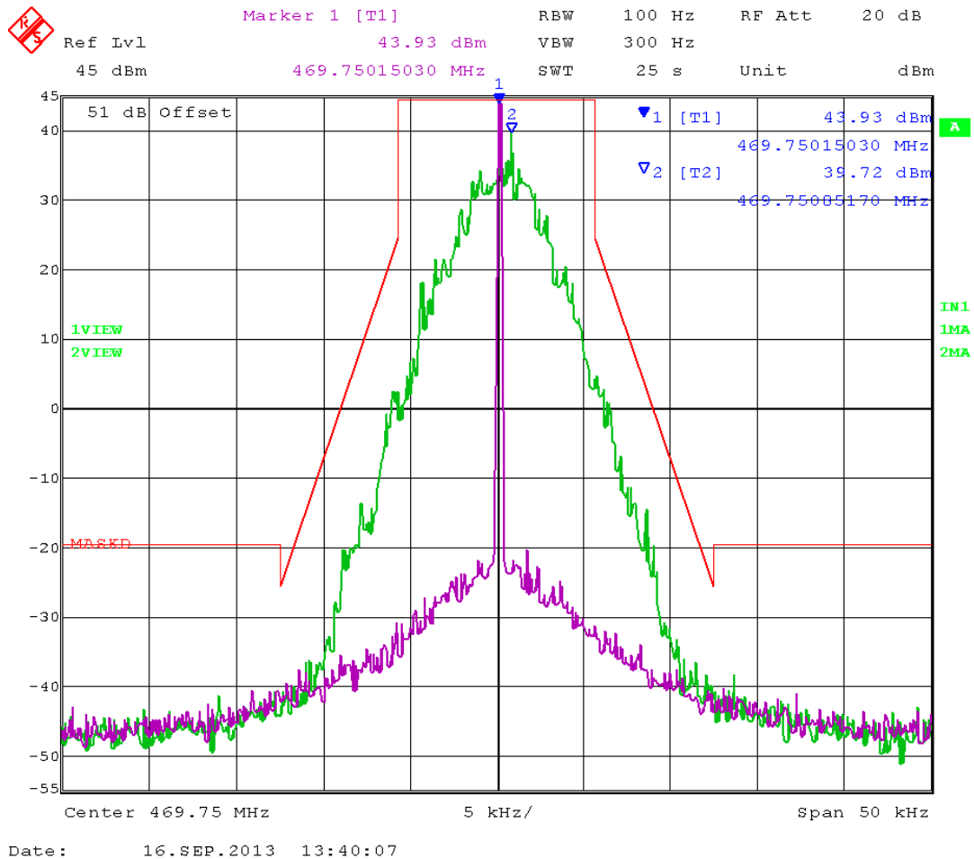
Figure 8: Occupied bandwidth 469.75 MHz (12.5 kHz-digital)
