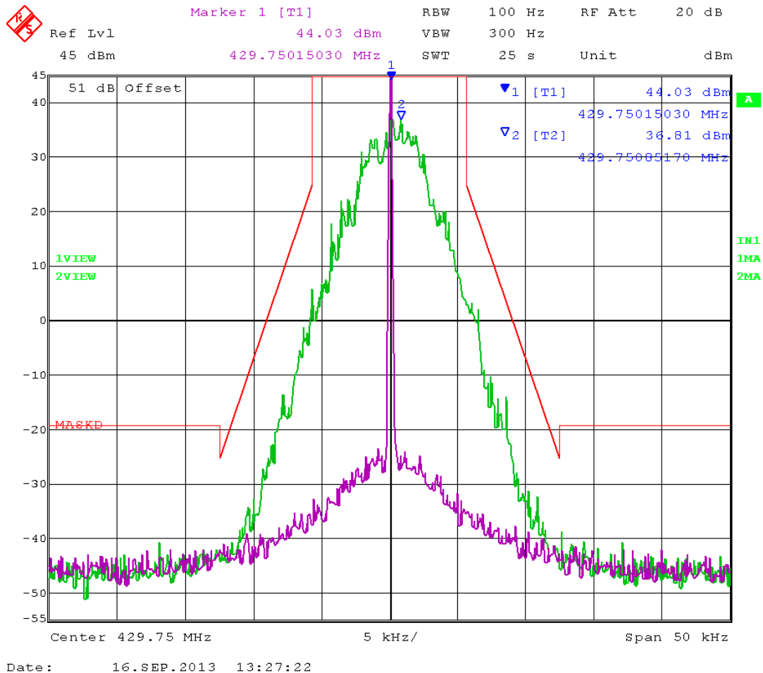
Figure 6: Occupied bandwidth 429.75 MHz (12.5 kHz-digital)
