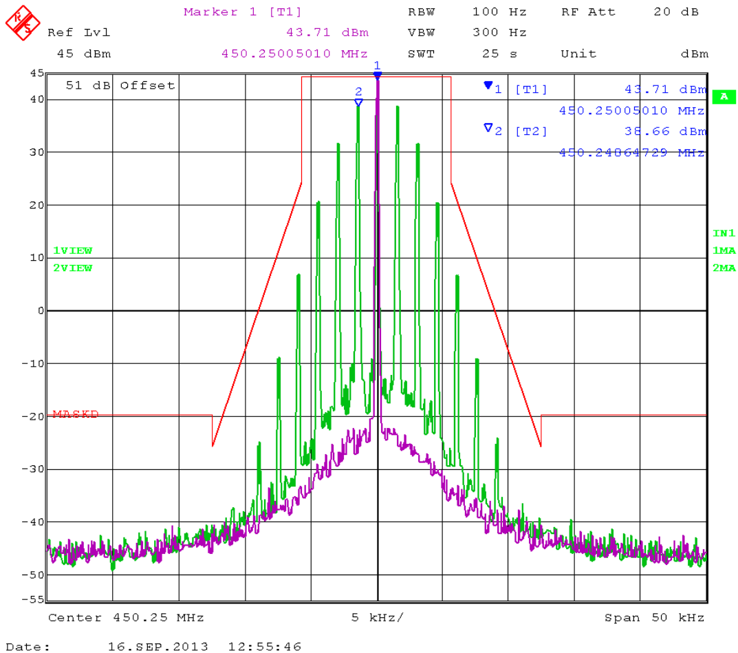
Figure 3: Occupied bandwidth 450.25 MHz (12.5 kHz)
