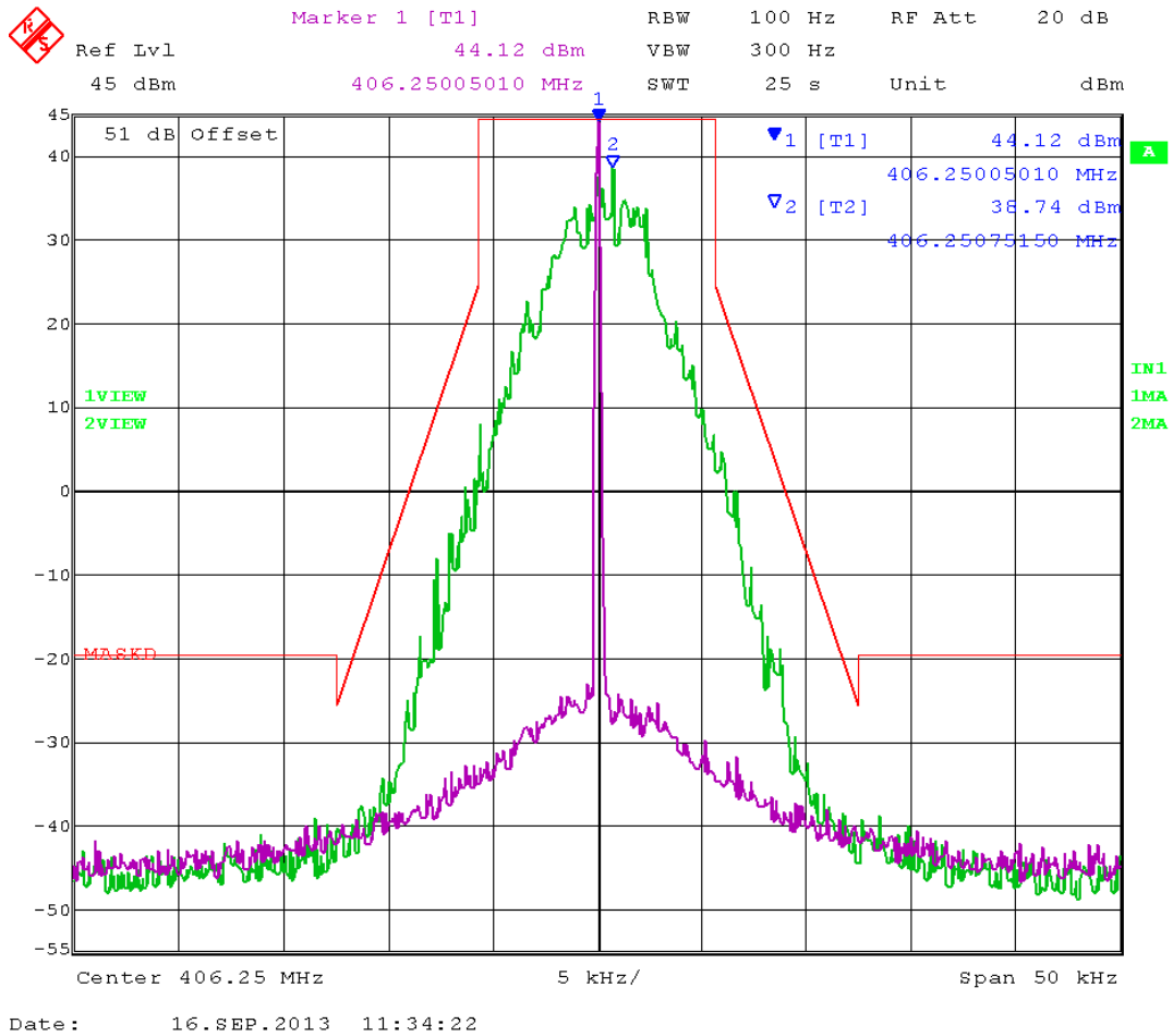
Figure 5: Occupied bandwidth 406.25 MHz (12.5 kHz-digital)
