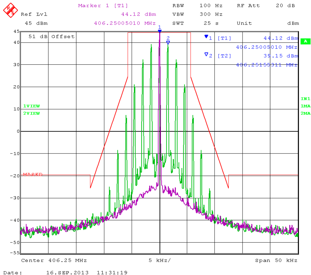
Figure 1: Occupied bandwidth 406.25 MHz (12.5 kHz)
