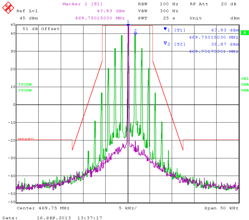
Figure 4: Occupied bandwidth 469.75 MHz (12.5 kHz)
