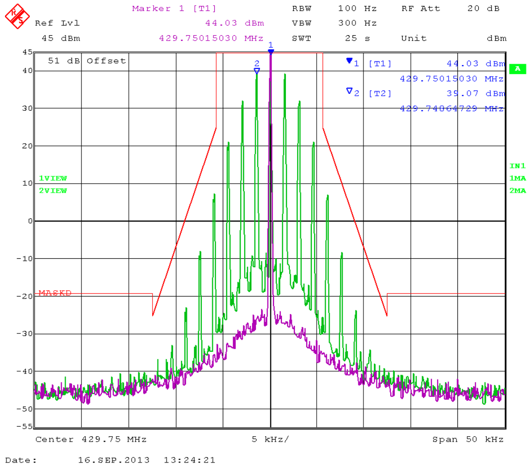
Figure 2: Occupied bandwidth 429.75 MHz (12.5 kHz)
