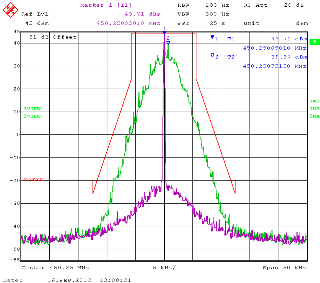
Figure 7: Occupied bandwidth 450.25 MHz (12.5 kHz-digital)
