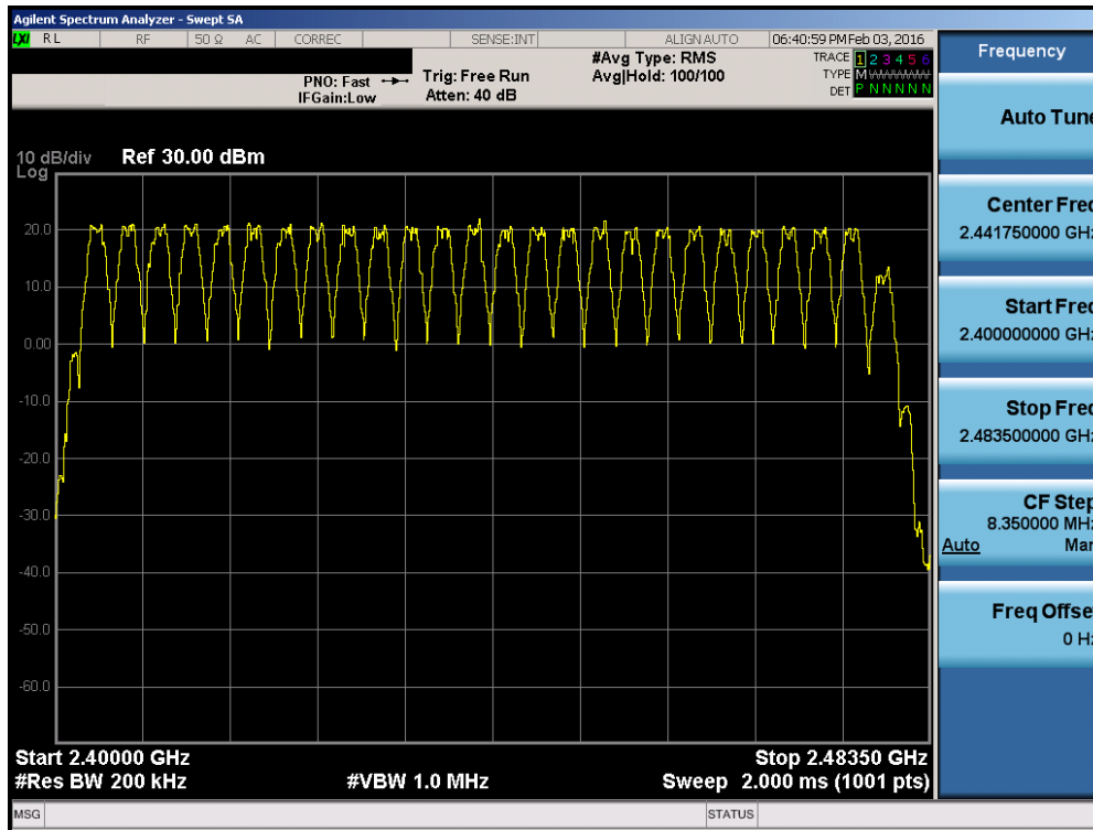
Plot 7-17. 2400MHz Spectrum Channel Hopping Plot (2400 MHz Band)
