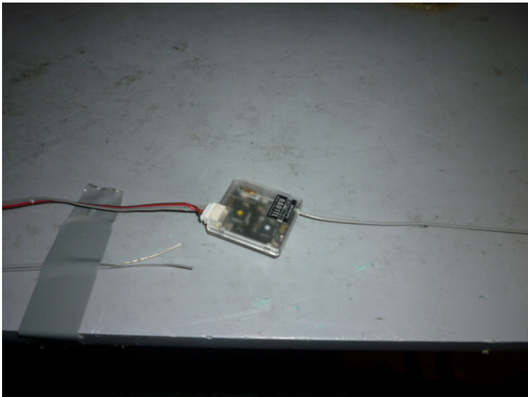
Set-up for Radiated Emission (Transceiver)
