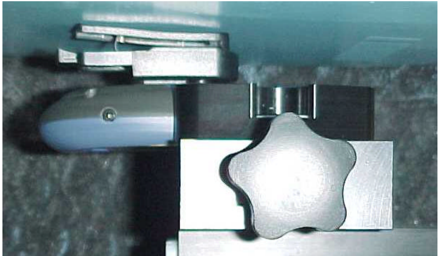
Position of device against flat phantom using carry accessory SXK –107-6820/55.
