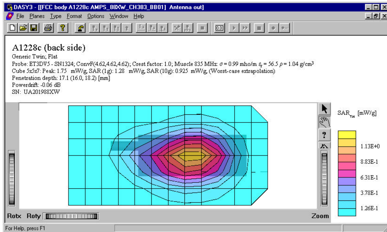
Distribution of maximum SAR in 800 AMPS band.
