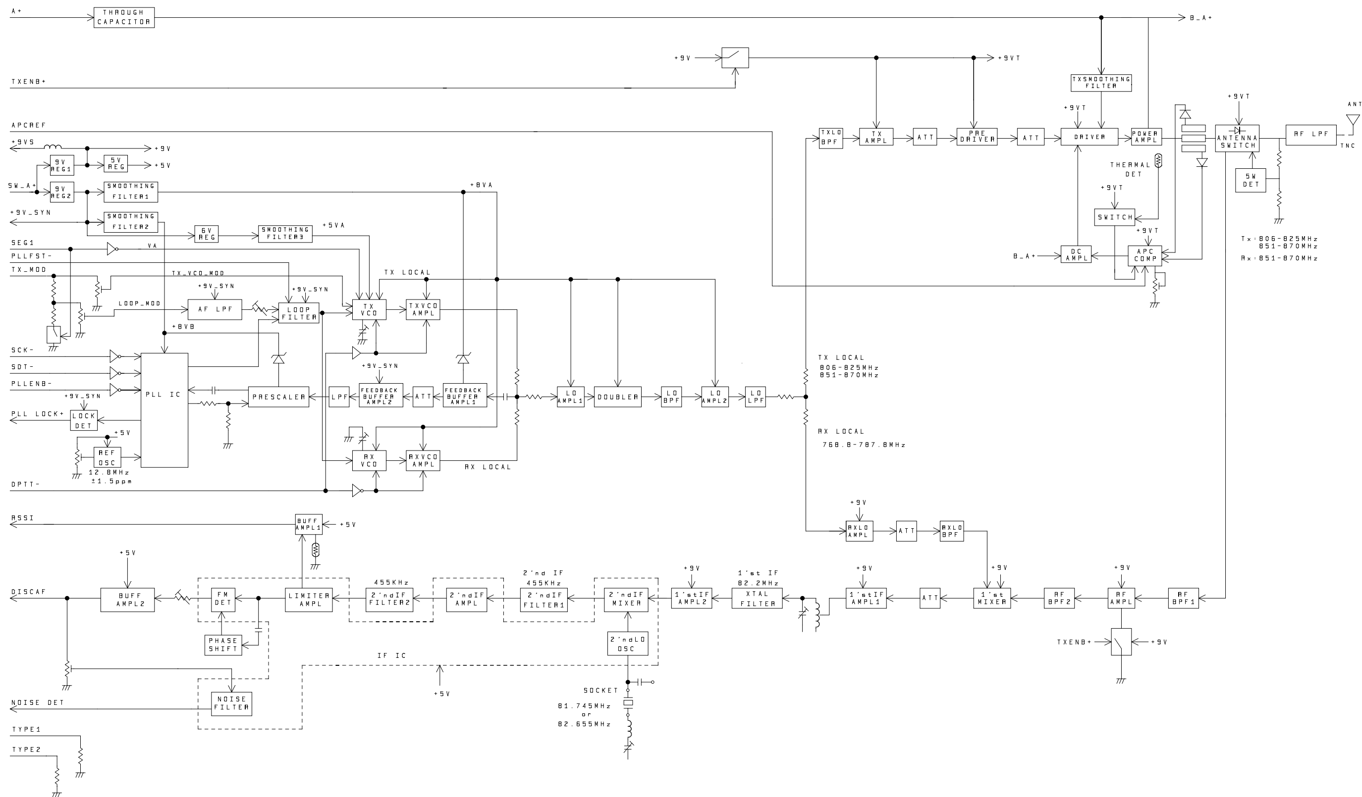
Block Diagram of KME800 TRX Board Unit For FCC XA00-TM-0186
