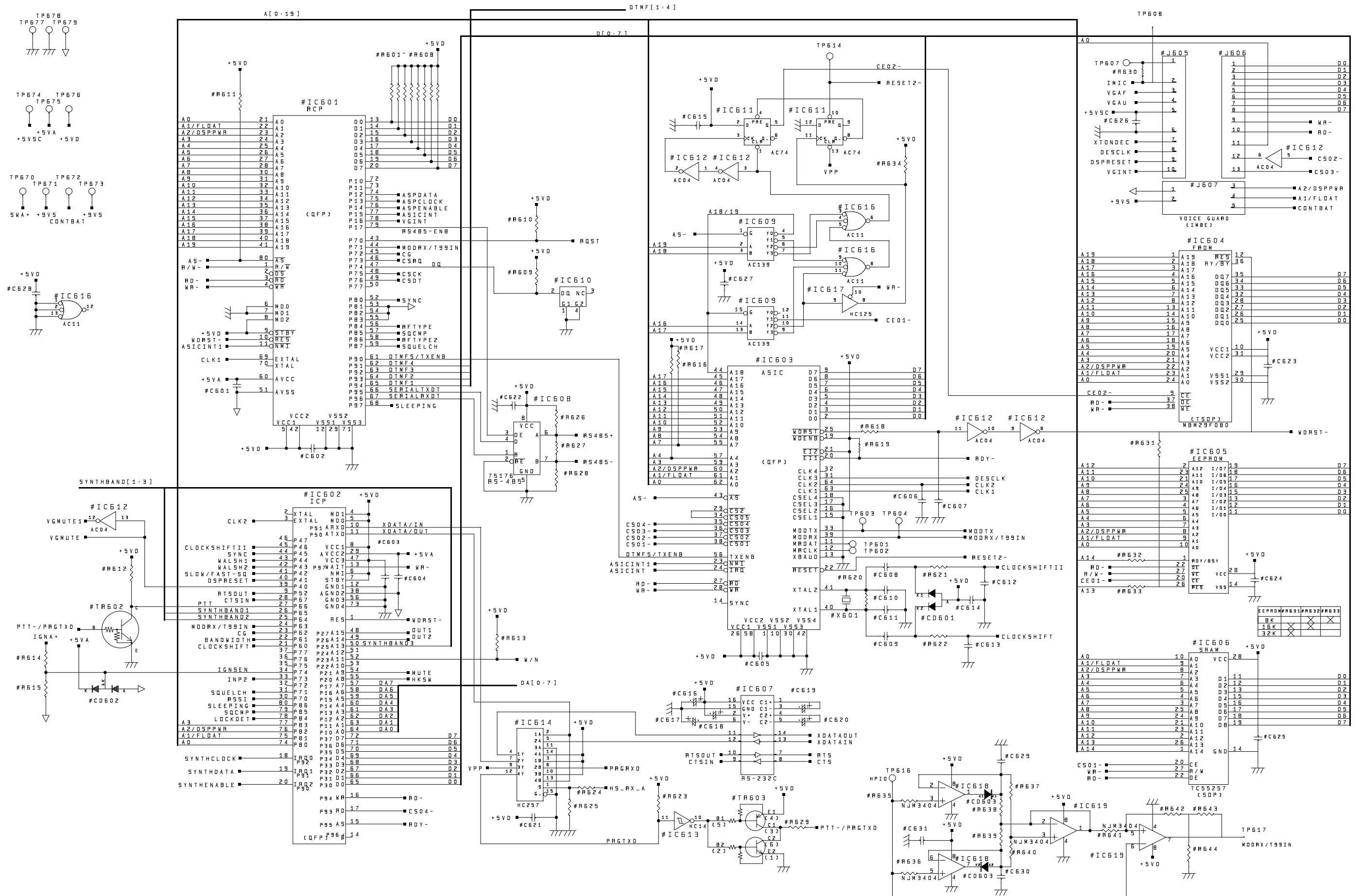
Schematic of KME System Control Unit For FCC
