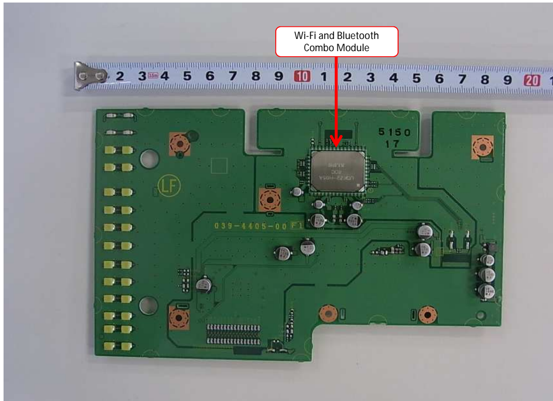
LCD PCB ASSY Component - F2 View
