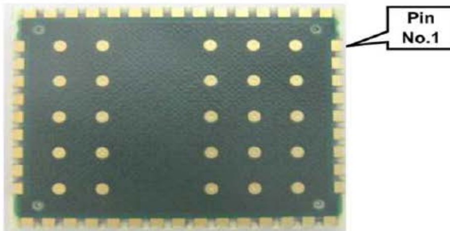
2.Bottom View
