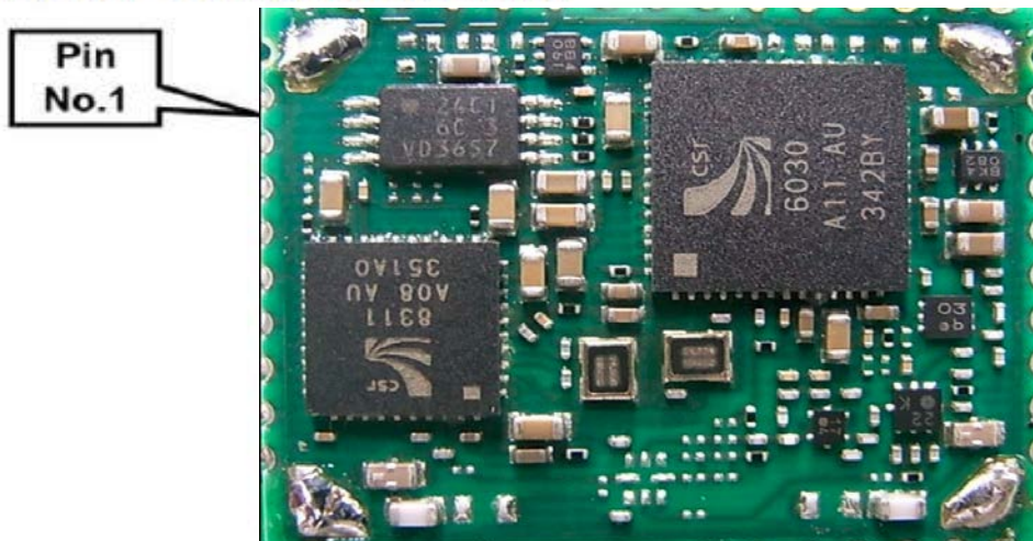
3.Top View - shielding case was removed
