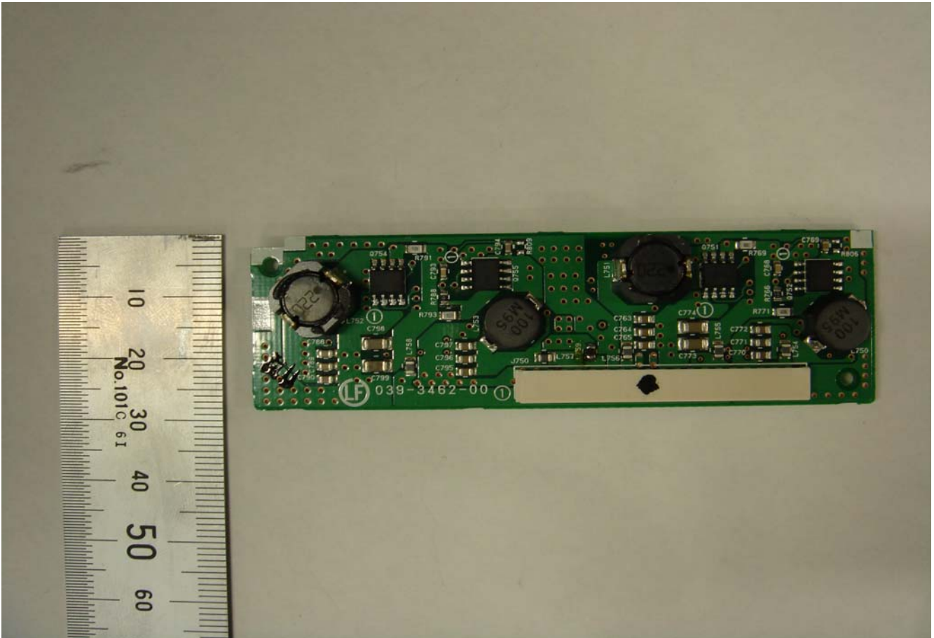
<Car Stereo DC/DC convertor PCB solder side>
