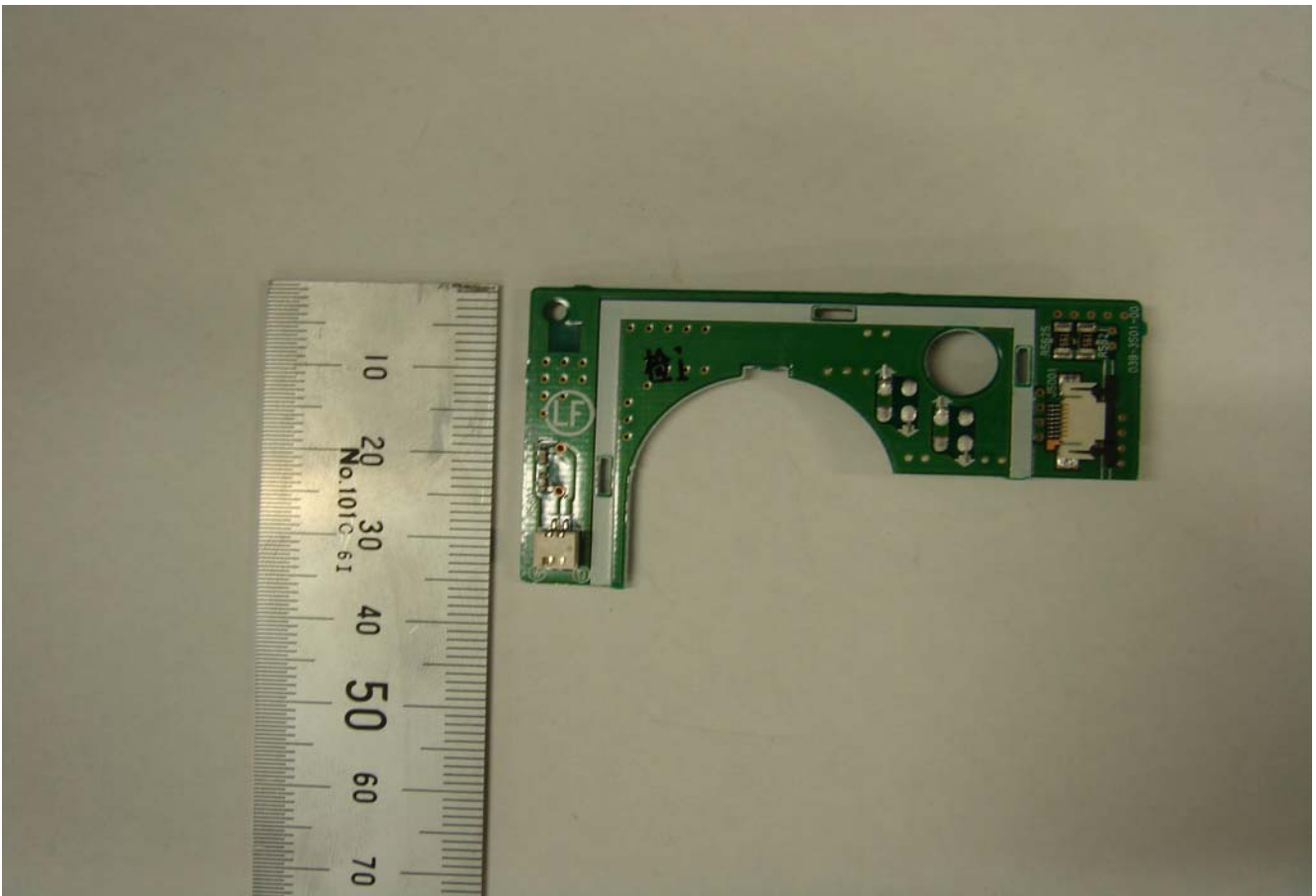
<Car Stereo Slide sensor PCB solder side>
