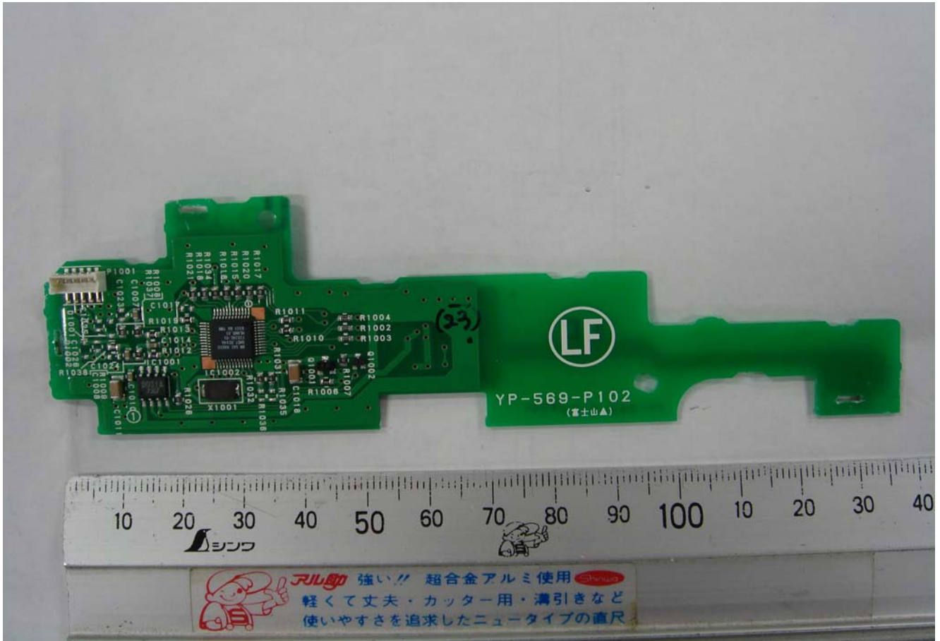
<Car Stereo XM Radio Control PCB solder side>
