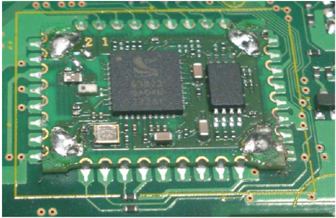
< Bluetooth Module without shield >
