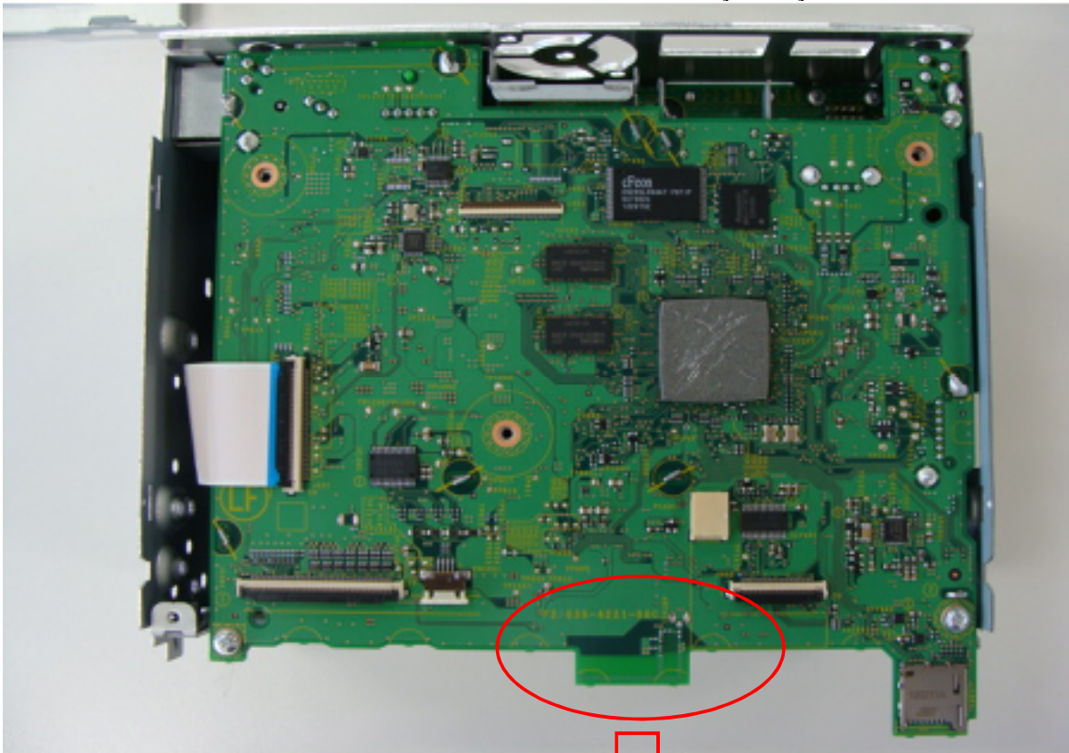
<Bluetooth RF Antenna on CPU PCB Assy F2 layer>
