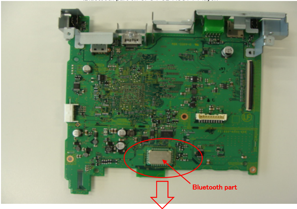
<Bluetooth part on CPU PCB ASSY F1 layer>
